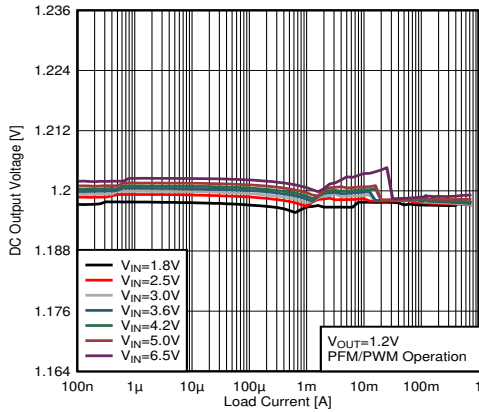
Figure 26. Output Voltage versus Load Current V OUT = 1.2 V
