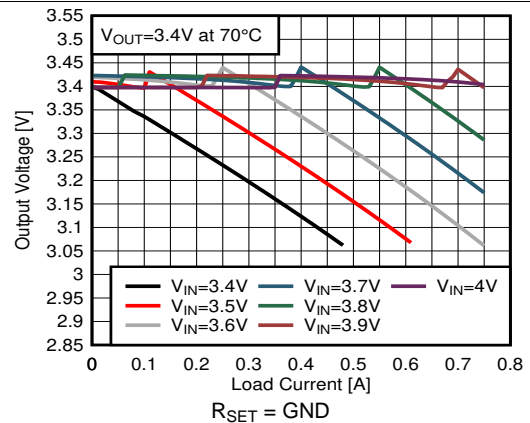
Figure 31. Output Voltage versus Load Current V OUT = 3.4 V
