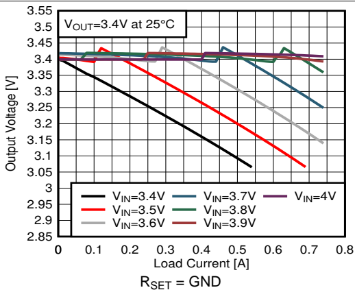
Figure 30. Output Voltage versus Load Current V OUT = 3.4 V
