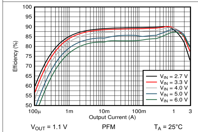
Figure 9-6. Efficiency Versus Output Current
