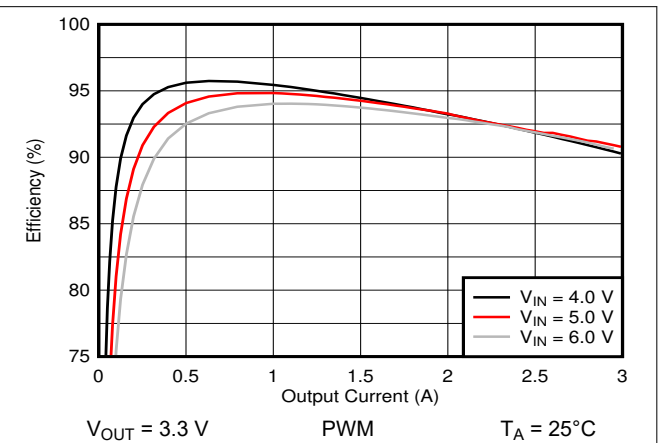
Figure 9-3. Efficiency Versus Output Current
