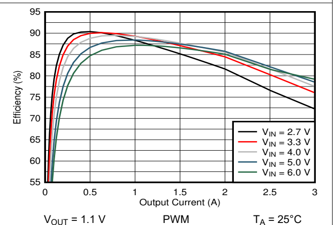
Figure 9-7. Efficiency Versus Output Current
