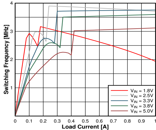
Figure 9-8. Switching Frequency
