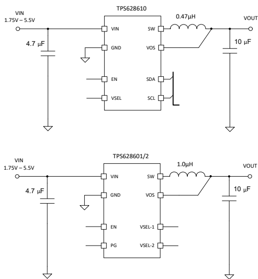
Typical Application
