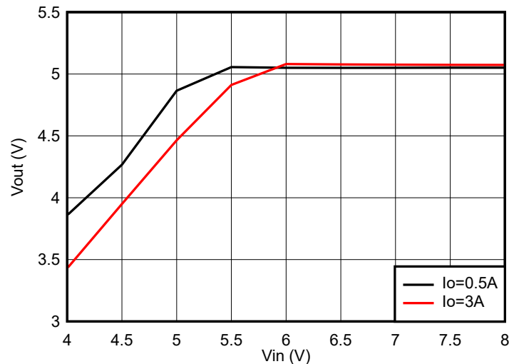
Figure 9-9. Overall Dropout Characteristic, V_{OUT} = 5\text{ V}
