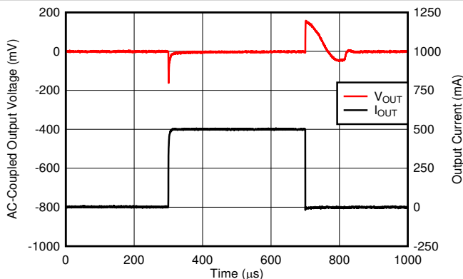
Figure 6-21. I_{OUT} Transient
