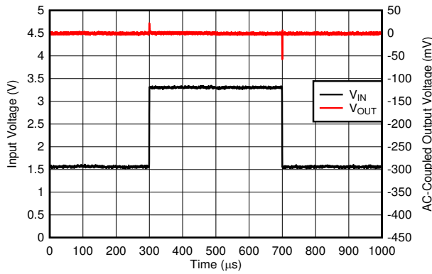
Figure 6-19. V_{IN} Transient
