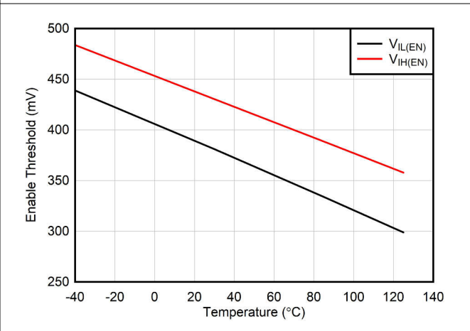
Figure 6-10. Enable Threshold vs Temperature
