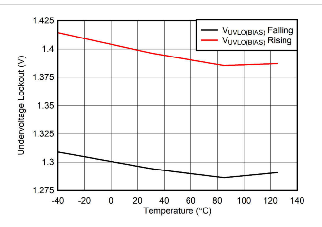
Figure 6-12. V_{\text{BIAS}} UVLO vs Temperature
