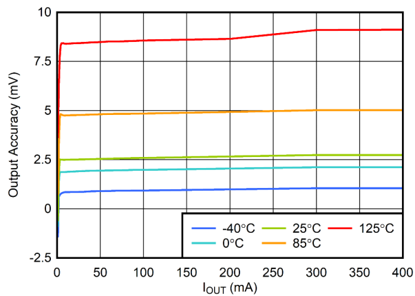
Figure 6-3. Output Voltage Accuracy vs I_{OUT}
