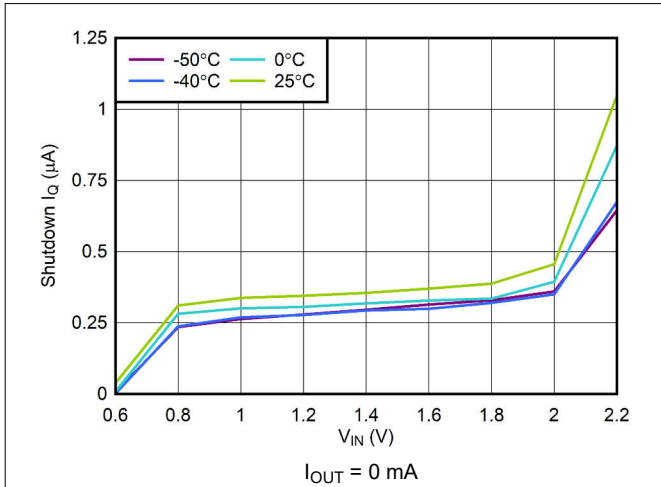
Figure 6-7. V_{\text{IN}} Shutdown I_{\text{Q}} vs V_{\text{IN}}
