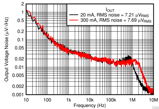
Figure 5-70. Noise vs Frequency and I_{OUT}
