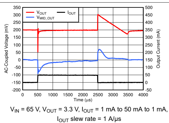
Figure 6-24. Load Transient
