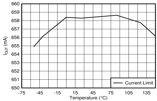
Figure 6-26. Output Current Limit vs Temperature
