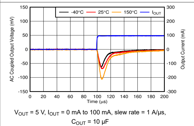
Figure 6-16. Load Transient, No Load to 100-mA Rising Edge
