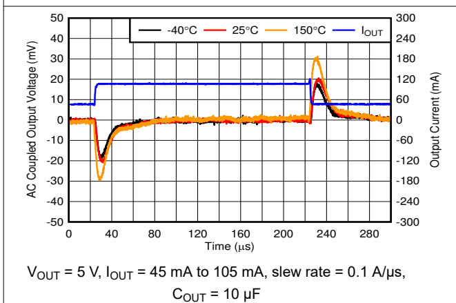
Figure 6-17. Load Transient, 45 mA to 105 mA
