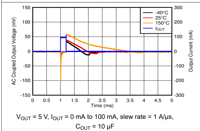
Figure 6-15. Load Transient, No Load to 100 mA
