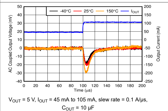
Figure 6-18. Load Transient, 45-mA to 105-mA Rising Edge
