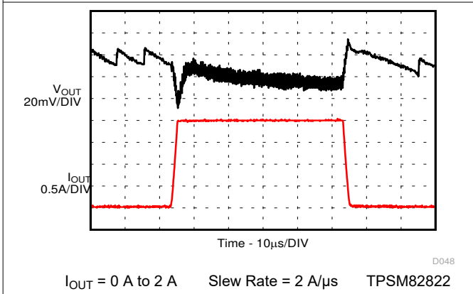
Figure 9-79. Load Transient
