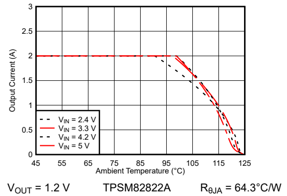
Figure 9-95. Safe Operating Area
