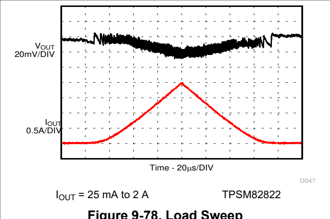
Figure 9-78. Load Sweep
