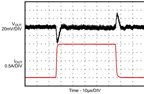
I_{OUT} = 0\text{ A to }2\text{ A} Slew Rate = 2 A/µs TPSM82822A
