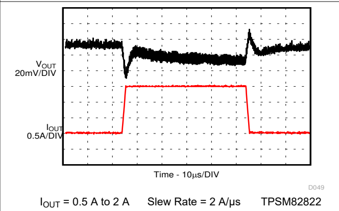
Figure 9-80. Load Transient
