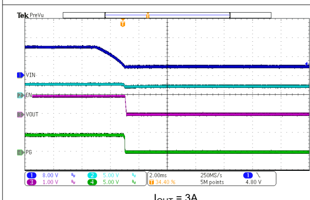
I_{OUT} = 3A Figure 7-14. VIN Shutdown
