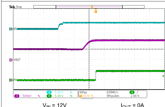
V_{IN} = 12V I_{OUT} = 0A Figure 7-12. EN Start-Up – 0.5V Prebias
