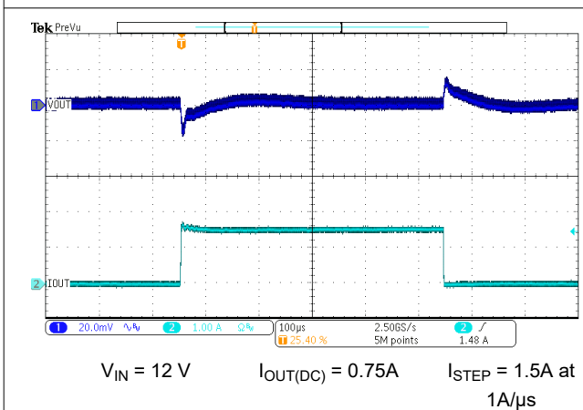
Figure 7-8. Load Transient
