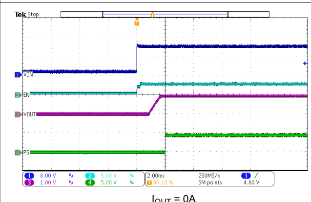
I_{OUT} = 0A Figure 7-13. VIN Start-Up
