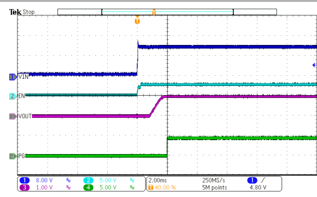
V_{IN} = 12V I_{OUT} = 6A Figure 7-11. EN Start-Up – With Load
