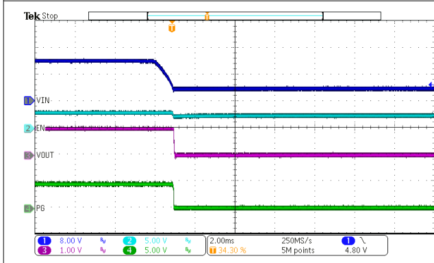
I_{OUT} = 6A Figure 7-14. VIN Shutdown
