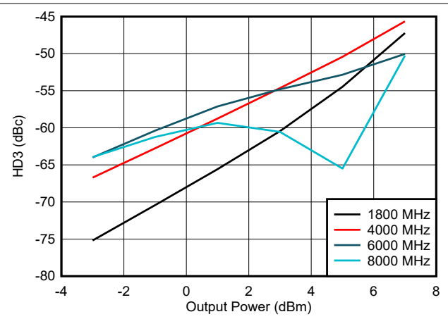
Figure 5-26. HD3 vs Output Power
