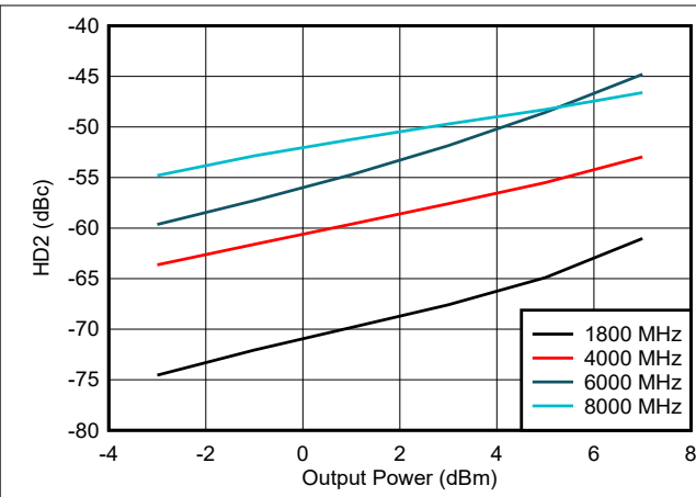
Figure 5-25. HD2 vs Output Power
