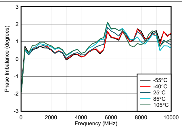
Figure 5-32. Phase Imbalance
