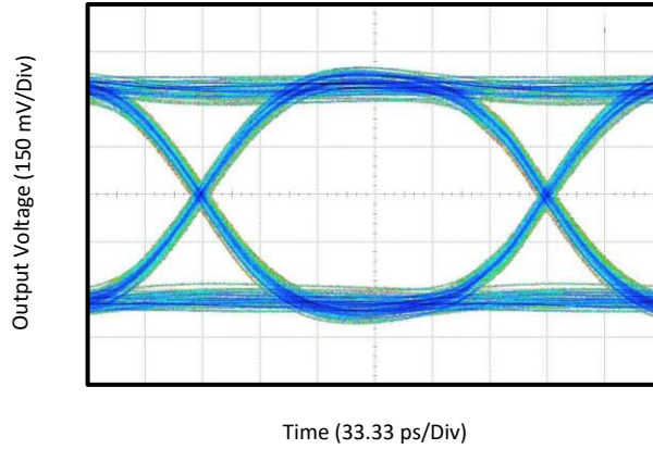
Figure 5-7. USB 3.2 Gen1 Eye-Pattern Performance with 12-inch Input PCB Trace at 5Gbps
