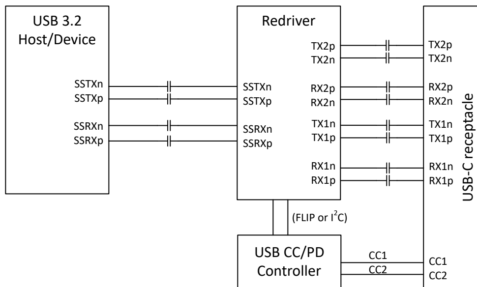
Simplified Schematic
