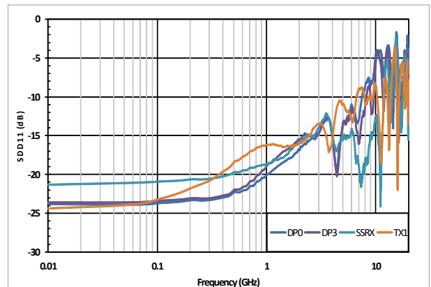
Figure 5-6. Output Return Loss Performance
