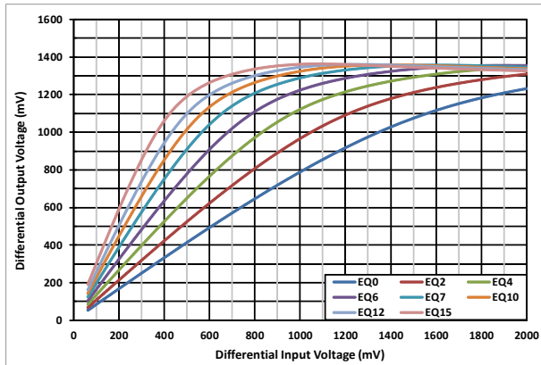
Figure 5-3. USB SSTX Linearity Curves at 2.5GHz
