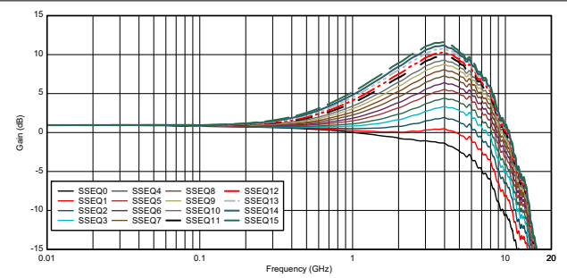
Figure 5-2. USB SSTX EQ Settings Curves
