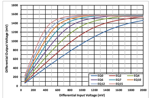
Figure 5-4. USB RX1 Linearity Curves at 2.5GHz
