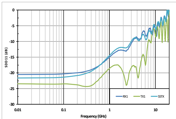
Figure 5-5. Input Return Loss Performance
