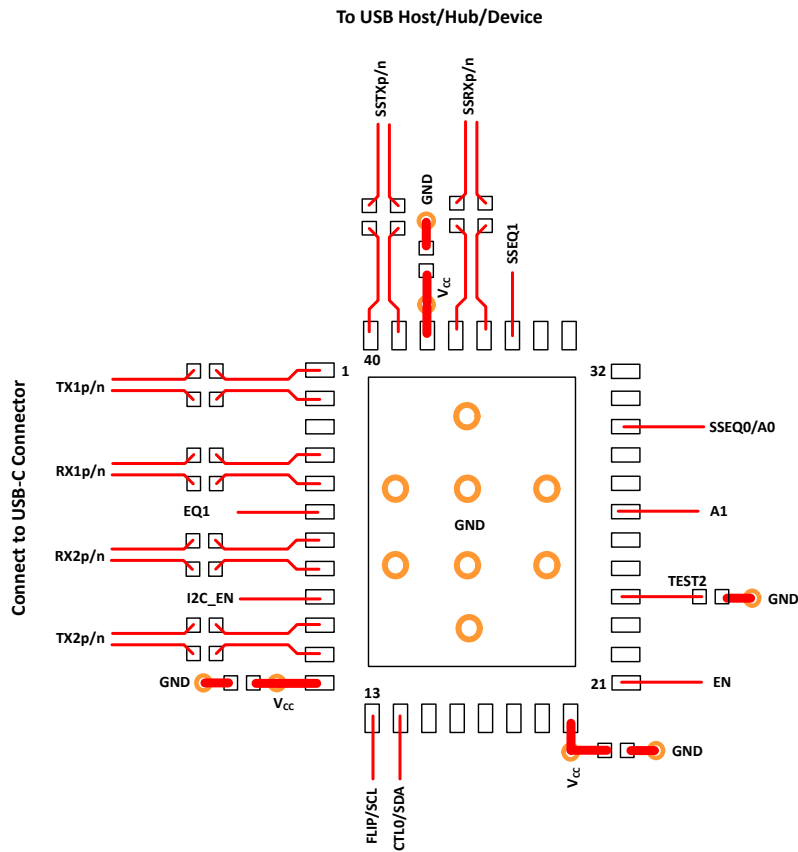
Figure 8-4. Layout Example
