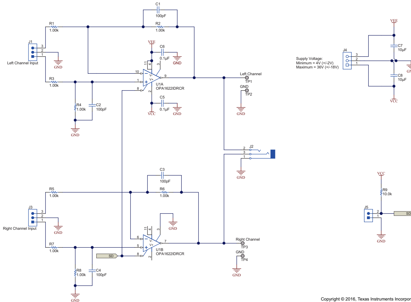
Figure 13. OPA1622EVM Schematic
