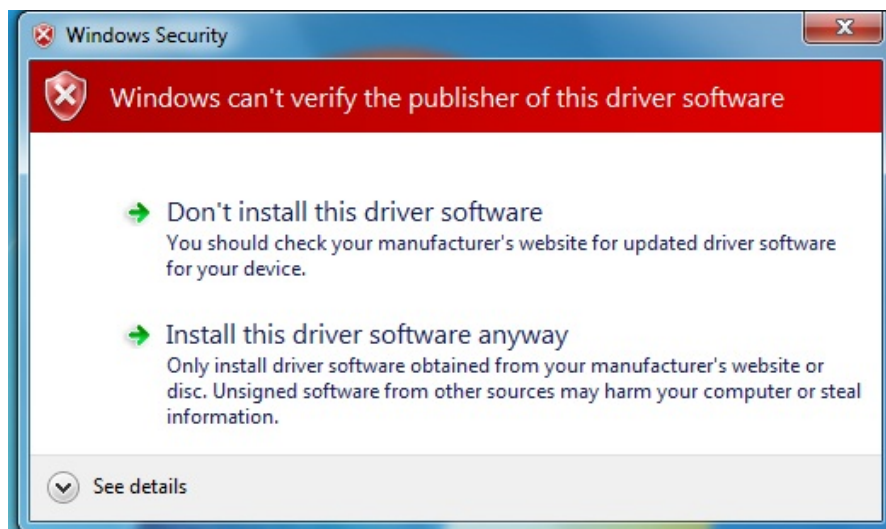
Figure 3. Windows Security
