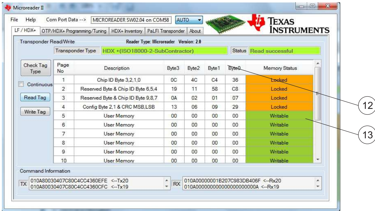
Figure 12. Read or Write Memory Content of HDX+ Transponder
