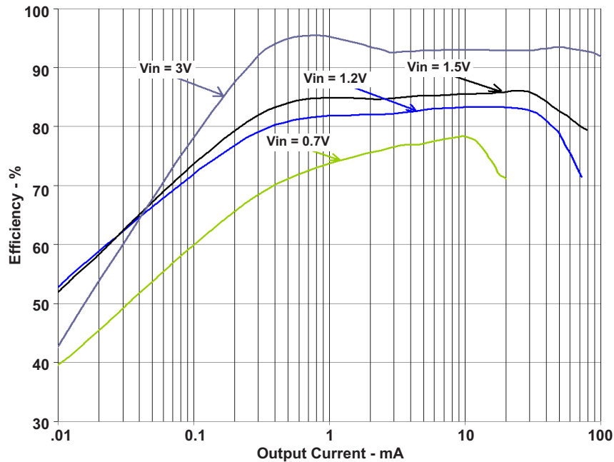
Figure 5. TLV61220 Efficiency
