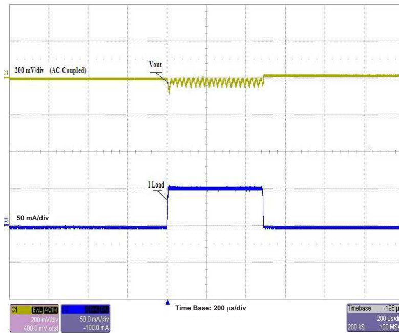
Figure 4. Load Transient
