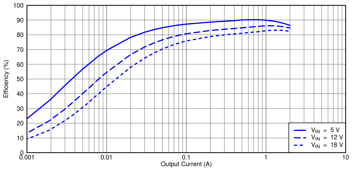
Figure 4-4. TPS54495EVM Converter 2 Light Load Efficiency
