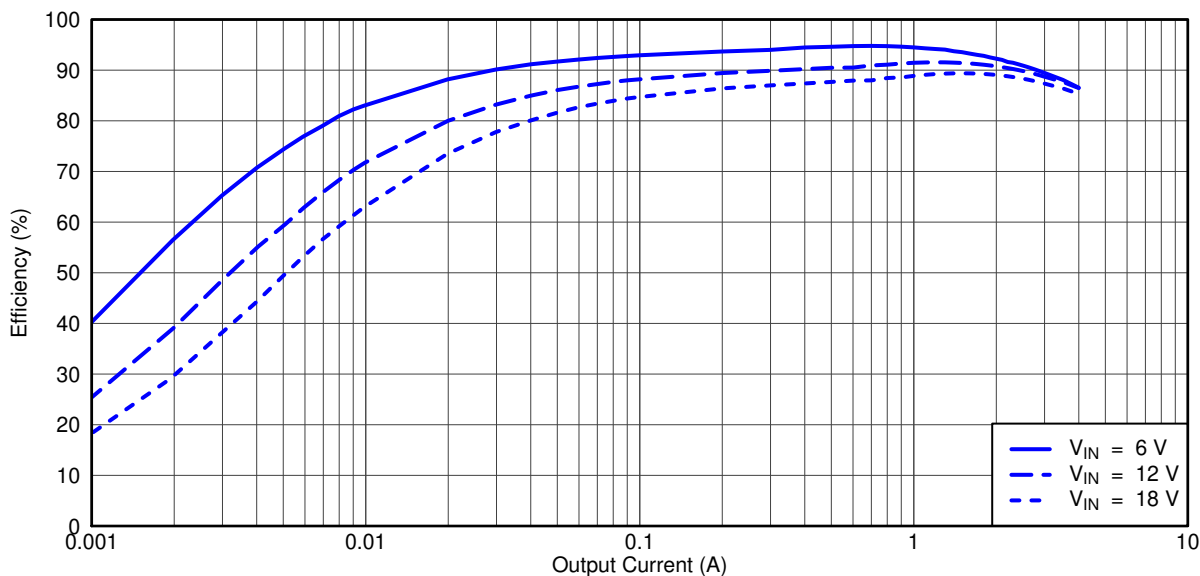
Figure 4-2. TPS54495EVM Converter 1 Light Load Efficiency
