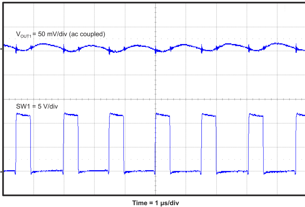
Figure 4-11. TPS54495EVM Converter 1 Output Voltage Ripple
