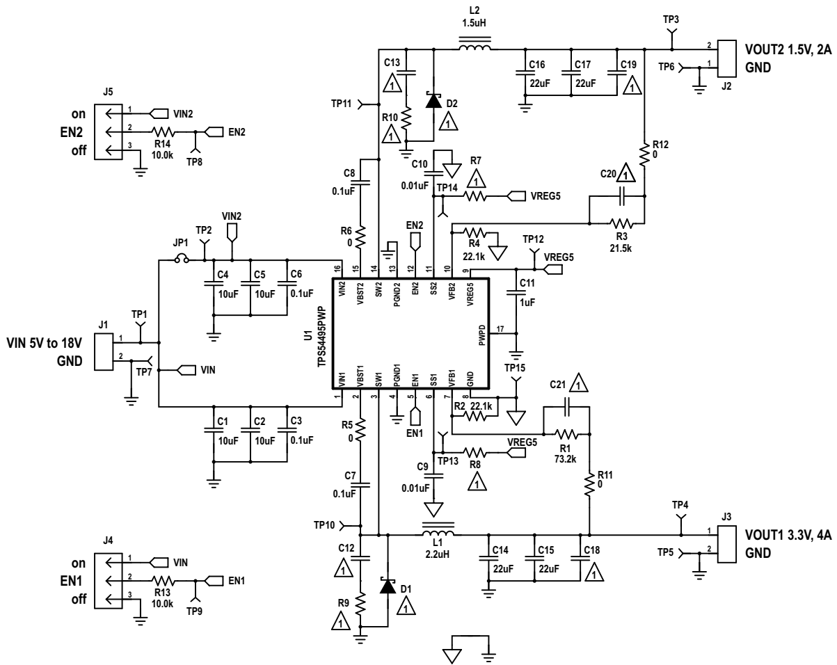
Figure 6-1. TPS54495EVm Schematic Diagram
