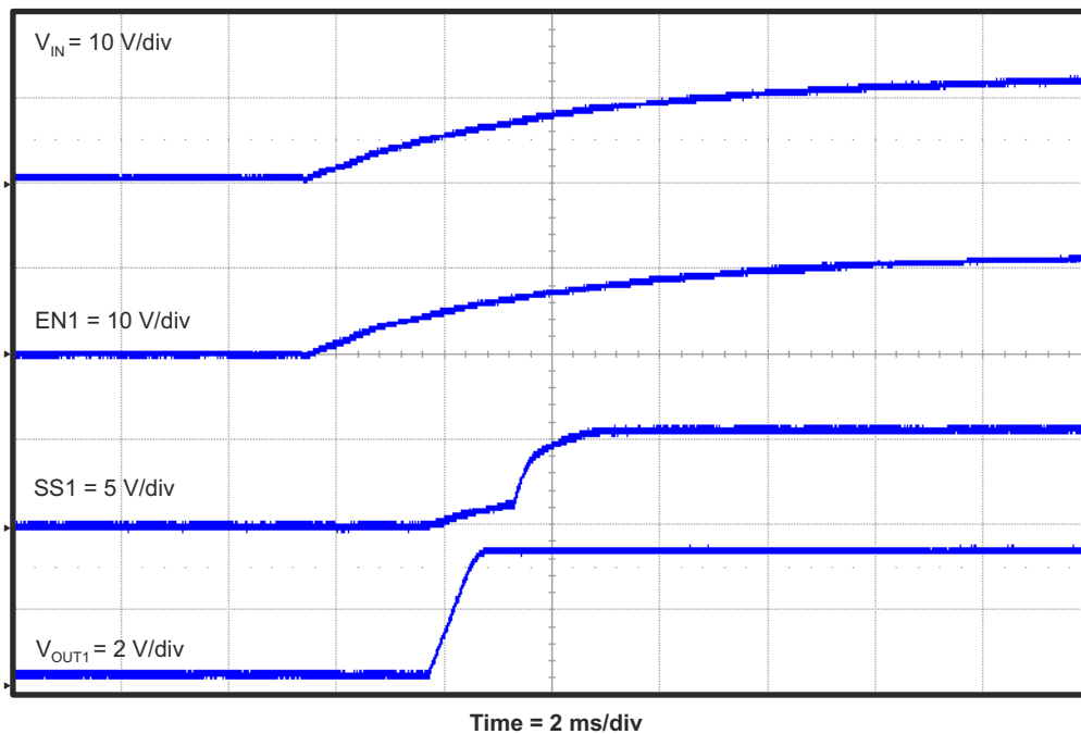
Figure 4-16. TPS54495EVM Converter 1 Start-Up Relative to V_{IN}
