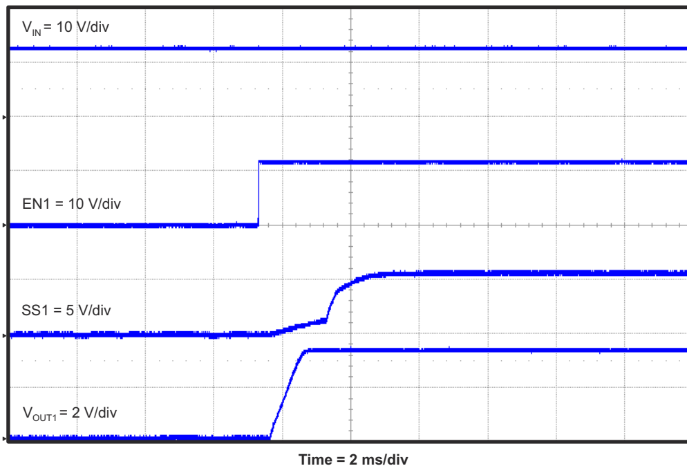
Figure 4-17. TPS54495EVM Start-Up Relative to EN1
