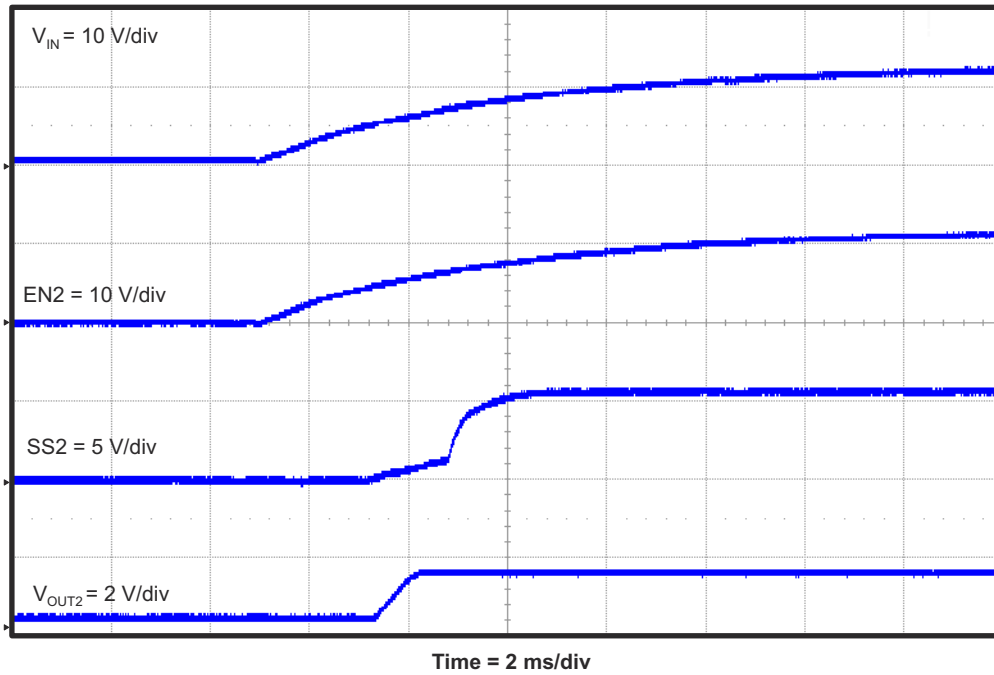
Figure 4-18. TPS54495EVM Converter 2 Start-Up Relative to V_{IN}
