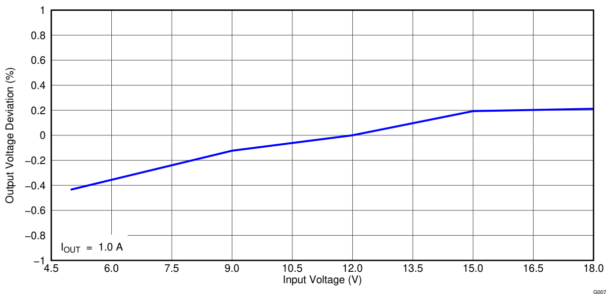
Figure 4-8. TPS54495EVM Converter 2 Line Regulation
