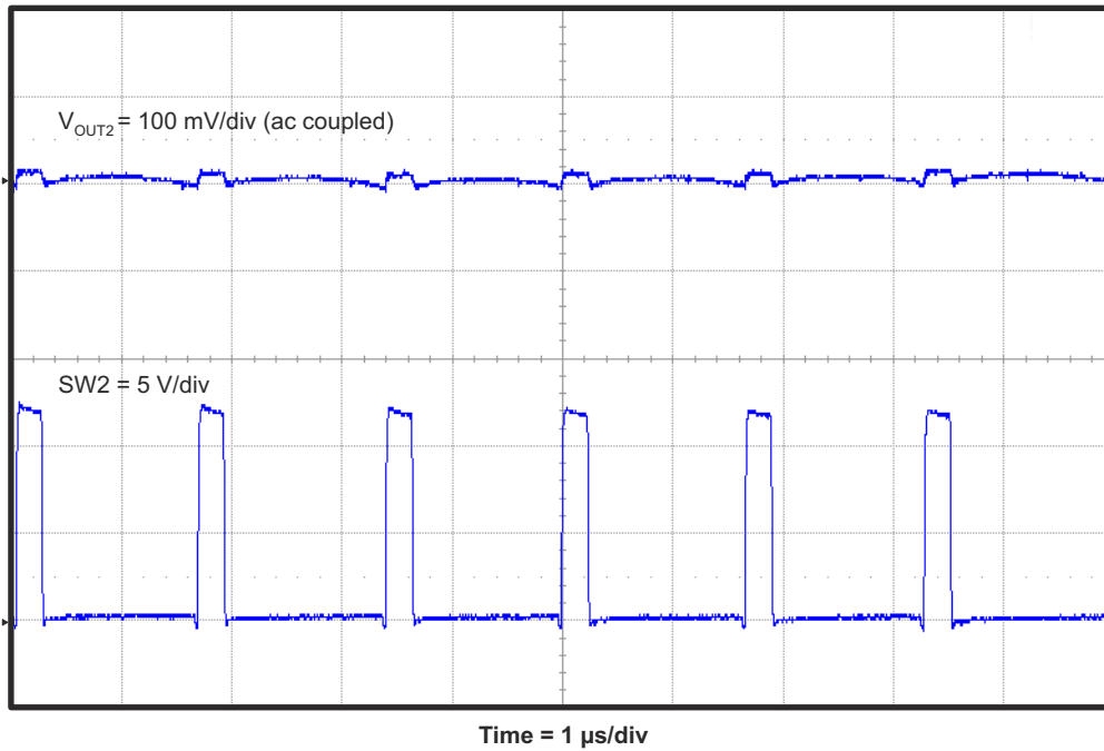
Figure 4-13. TPS54495EVM Converter 2 Output Voltage Ripple
