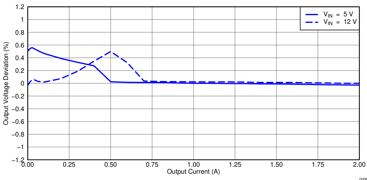
Figure 4-6. TPS54495EVM Converter 2 Load Regulation
