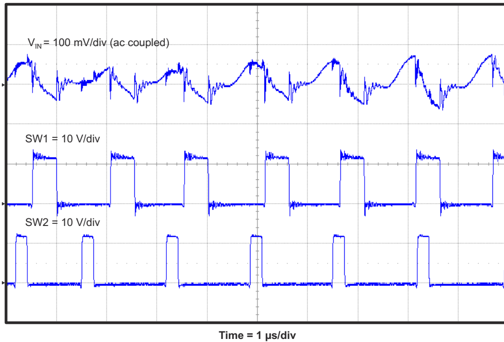
Figure 4-15. TPS54495EVM Input Voltage Ripple
