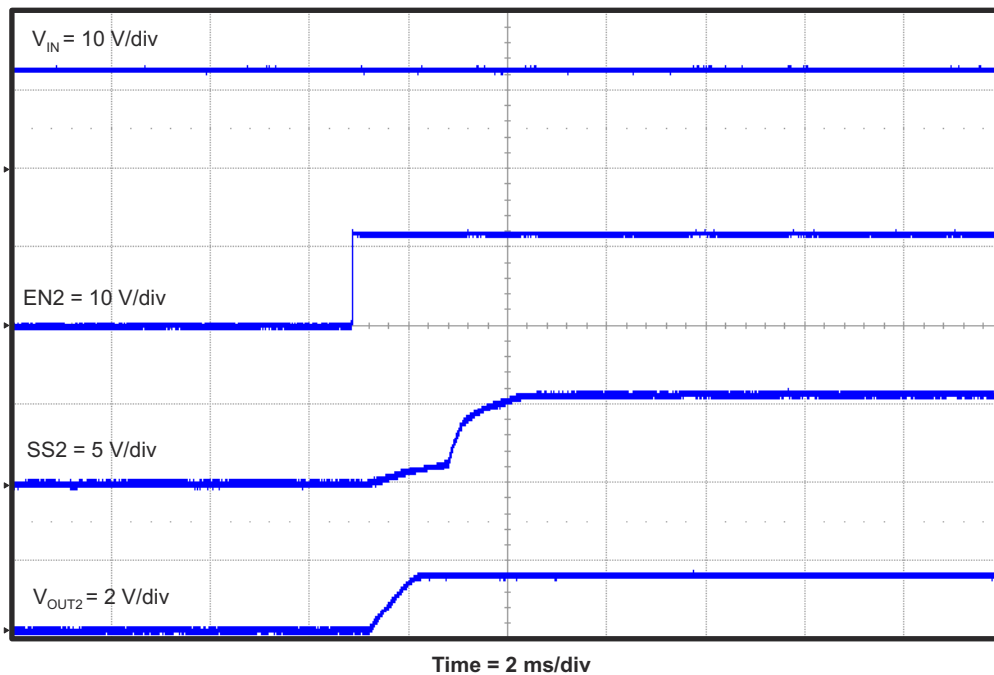
Figure 4-19. TPS54495EVM Start-Up Relative to EN2
