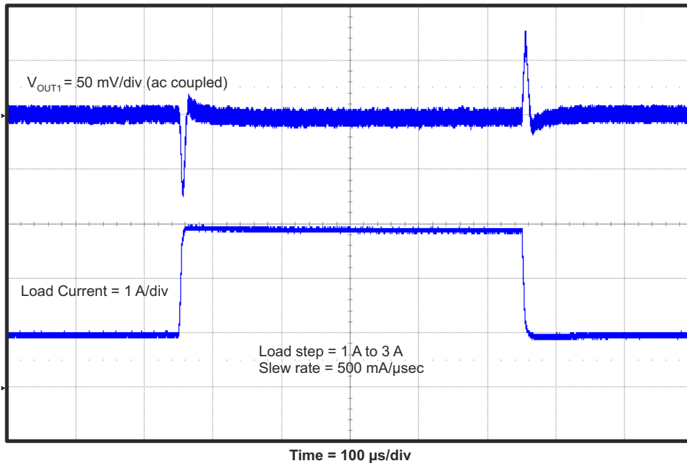
Figure 4-9. TPS54495EVM Converter 1 Load Transient Response
