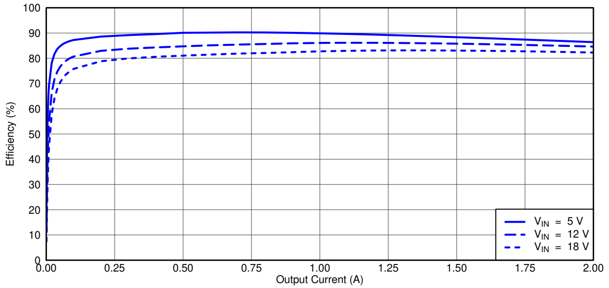
Figure 4-3. TPS54495EVM Converter 2 Efficiency
