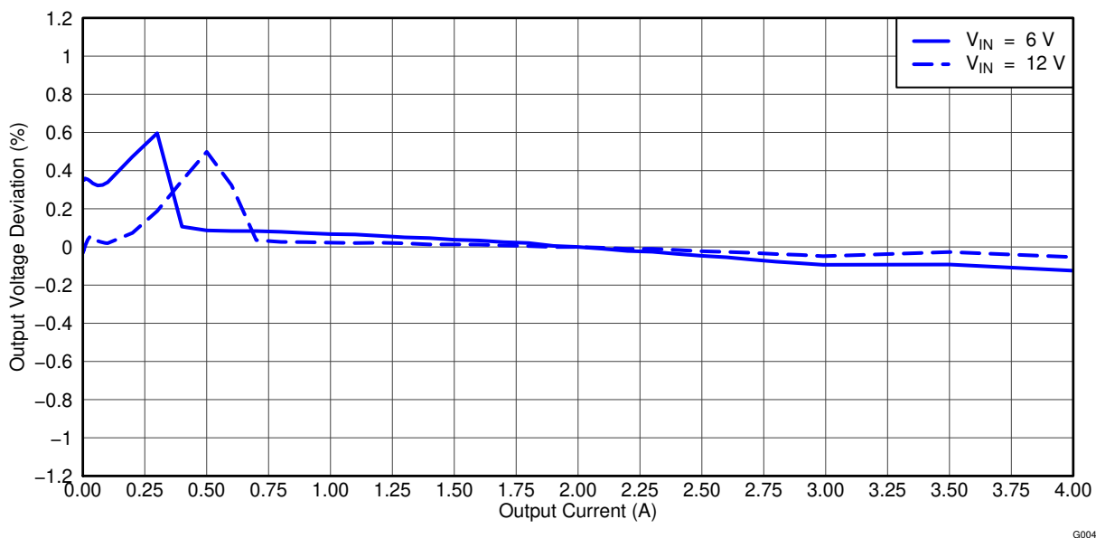
Figure 4-5. TPS54495EVM Converter 1 Load Regulation
