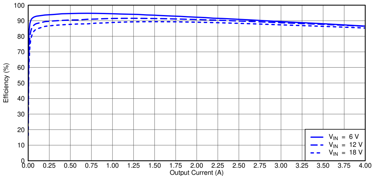
Figure 4-1. TPS54495EVM Converter 1 Efficiency
