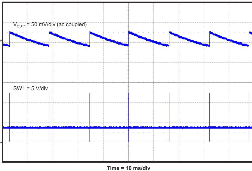
Figure 4-12. TPS54495EVM Converter 1 Eco-mode™ Output Voltage Ripple at No Load
