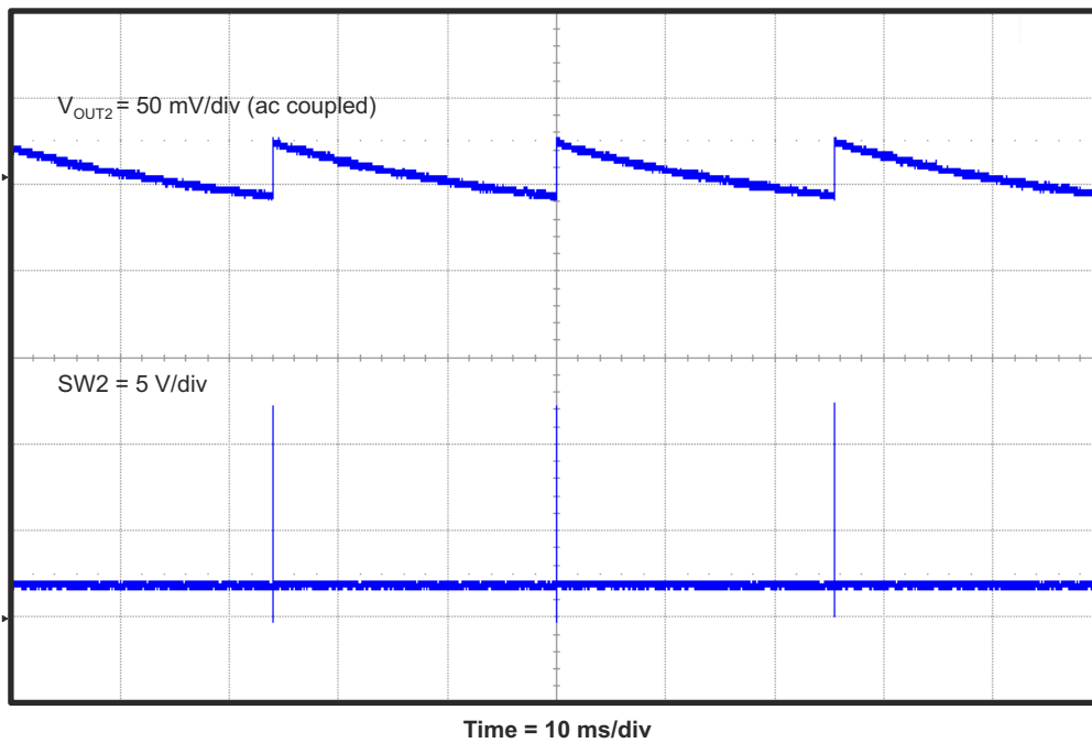
Figure 4-14. TPS54495EVM Converter 2 Eco-mode™ Output Voltage Ripple at No Load
