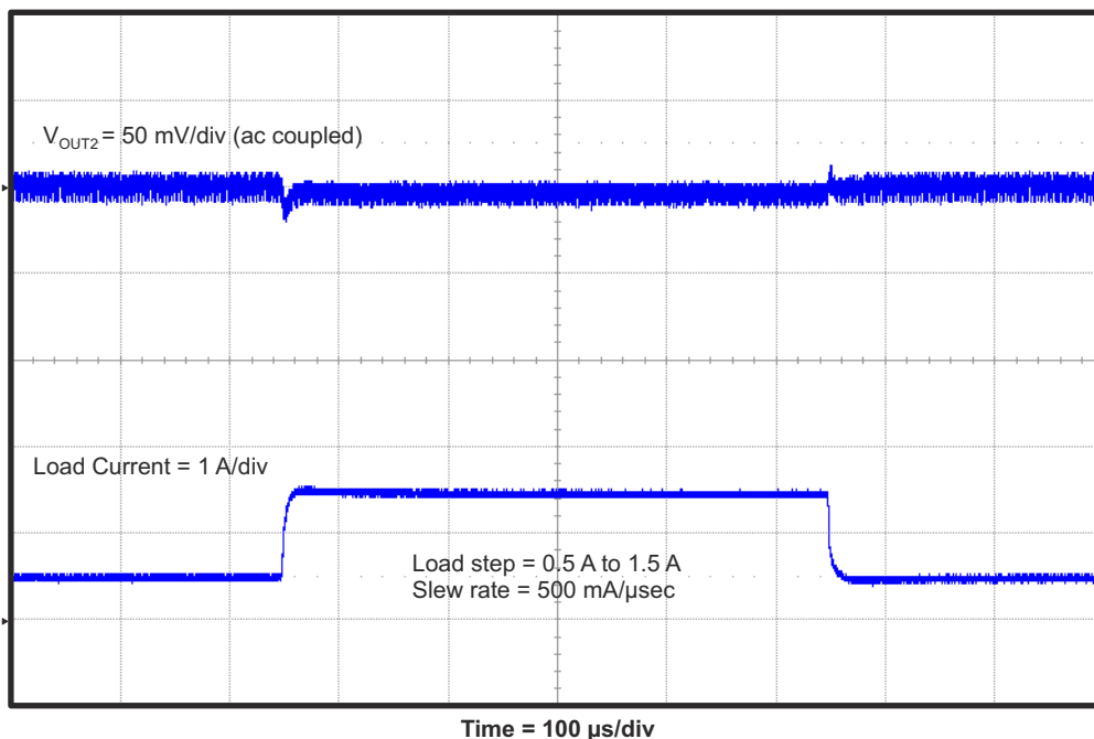
Figure 4-10. TPS54495EVM Converter 2 Load Transient Response
