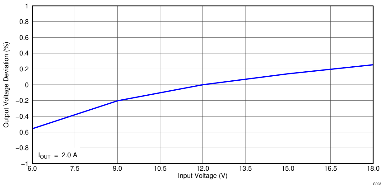
Figure 4-7. TPS54495EVM Converter 1 Line Regulation
