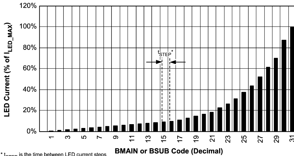
Figure 10. I_{MAIN} or I_{SUB} vs BMAIN or BSUB Data
