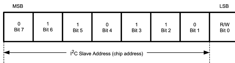
Figure 5. Chip Address
