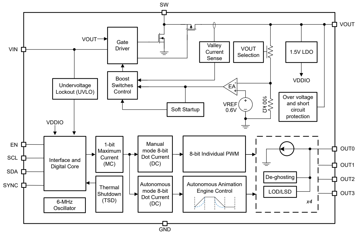
Figure 1-1. Device Block Diagram
