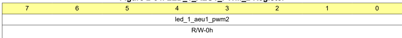
Figure 2-64. LED_1_AEU1_PWM_2 Register
