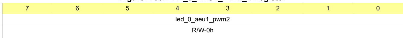
Figure 2-38. LED_0_AEU1_PWM_2 Register
