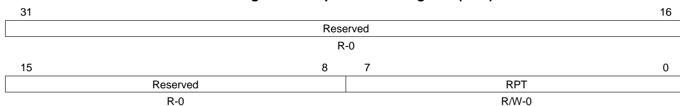
Figure 10. Repeat Count Register (RPT)
