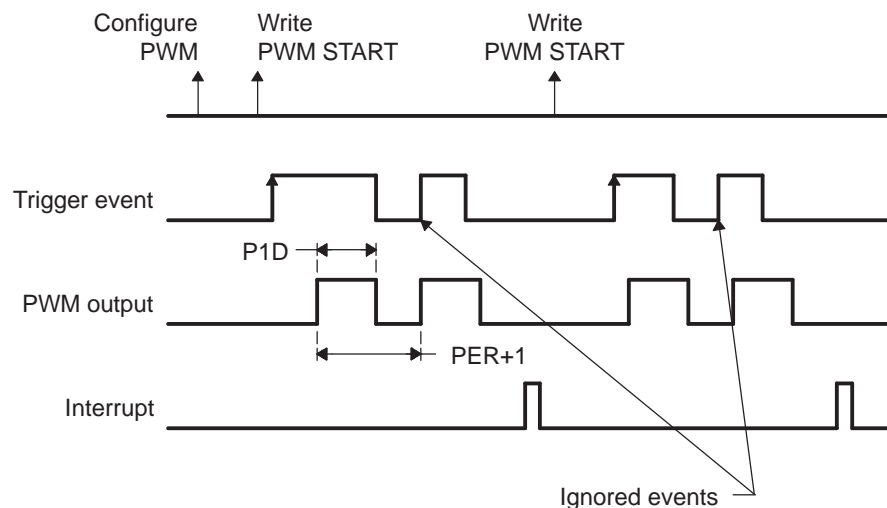
Figure 4. PWM Event-Triggered One-Shot Mode Operation (P1OUT = 1, INACTOUT = 0, EVTRIG = 1, PWM_RPT = 1)
