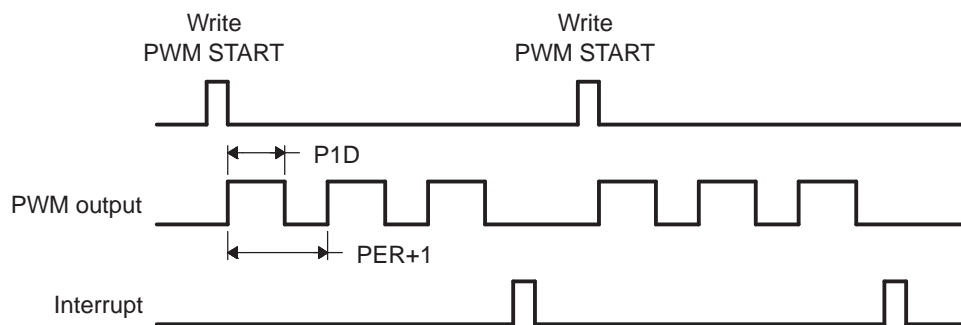
Figure 3. PWM One-Shot Mode Operation (P1OUT = 1, INACTOUT = 0, EVTRIG = 0, PWM_RPT = 2)
