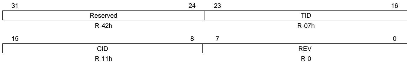
Figure 6. Peripheral Identification Register (PID)
