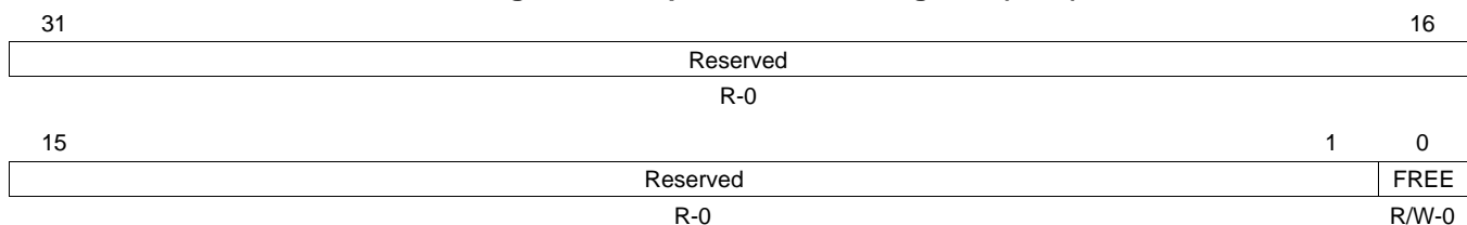
Figure 7. Peripheral Control Register (PCR)
