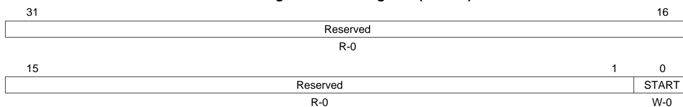
Figure 9. Start Register (START)
