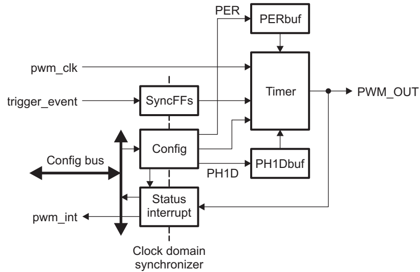
Figure 1. PWM Functional Block Diagram
