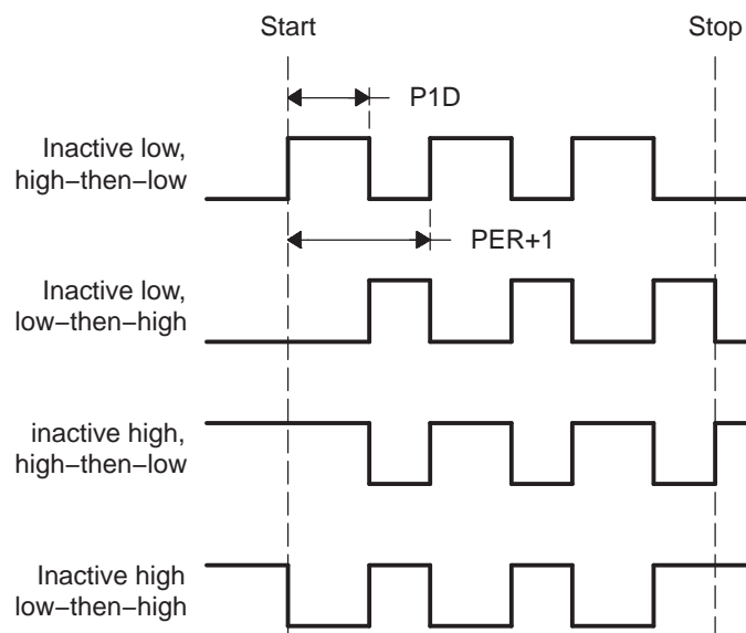
Figure 2. PWM Waveform Polarity Control (PWM_RPT = 2, for 3 periods)
