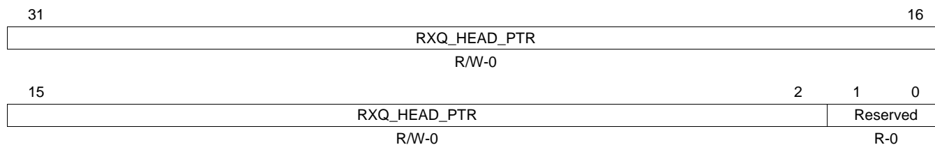
Figure 52. Receive CPPI DMA State Word 1 (RCPPIIDMASTATEW1)
