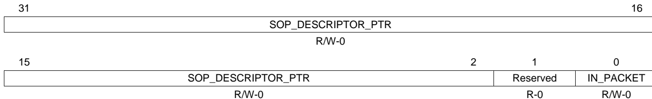
Figure 45. Transmit CPPI DMA State Word 1 (TCPPIDMASTATEW1)
