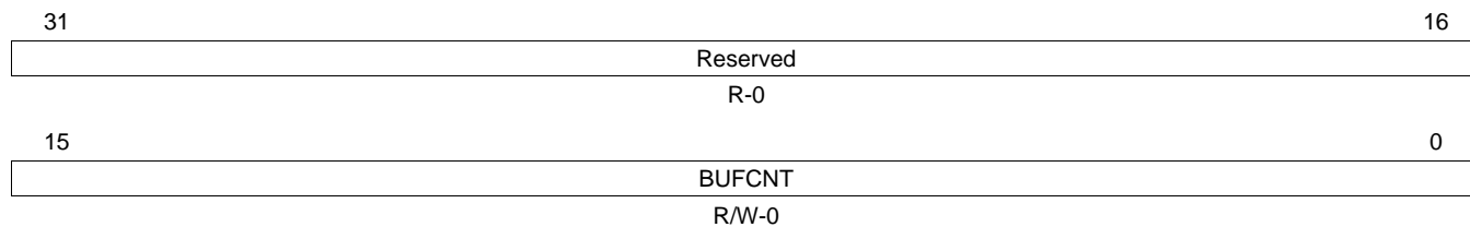
Figure 41. Receive Buffer Count 1 Register (RBUFCNT1)
