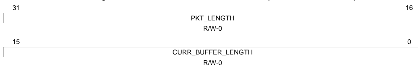
Figure 56. Receive CPPI DMA State Word 5 (RCPPIIDMASTATEW5)
