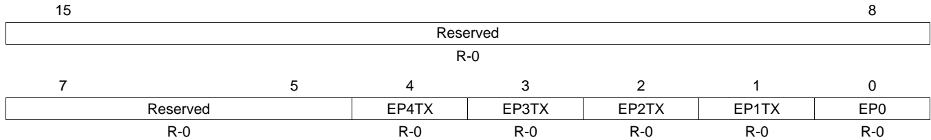
Figure 61. Interrupt Register for Endpoint 0 Plus Tx Endpoints 1 to 4 (INTRTX)
