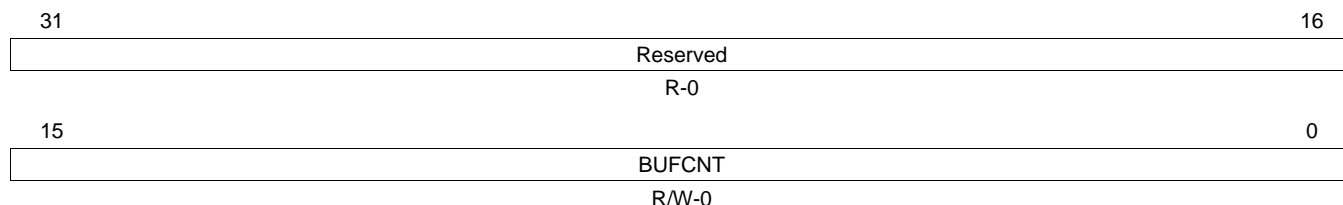
Figure 42. Receive Buffer Count 2 Register (RBUFCNT2)
