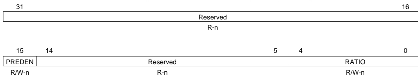
Figure 5. PLL Pre-Divider Register (PREDIV)
