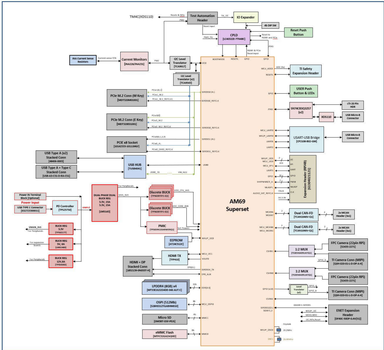
Figure 3-1. SK-AM69 Functional Block Diagram
