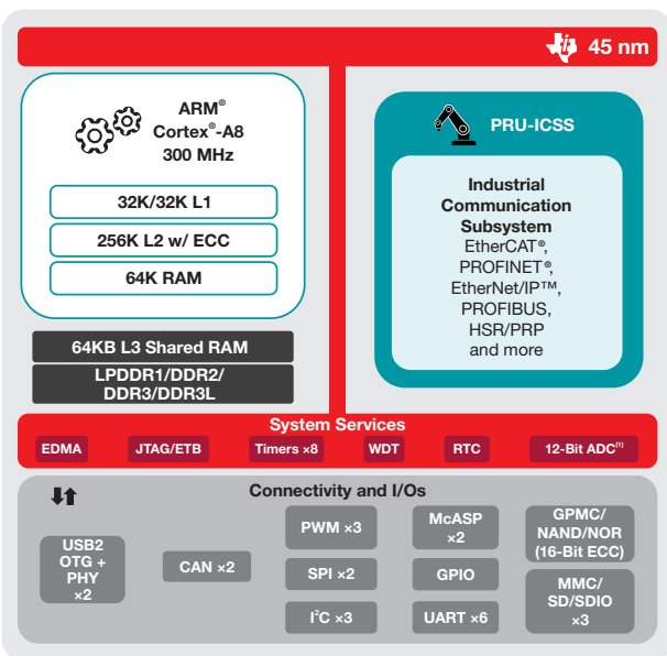
Figure 4: AMIC110 block diagram.
