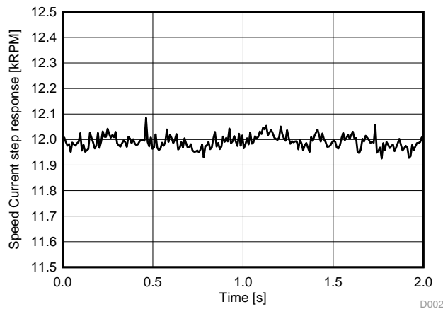
Figure 16. 12-kRPM Speed Stability Performance With Propeller
