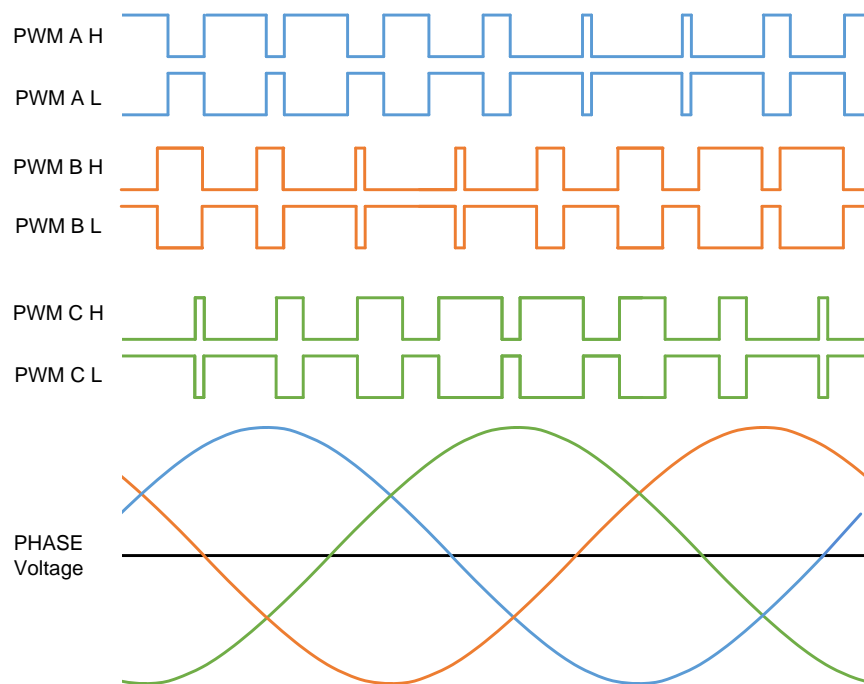
Figure 2. Generation of Ideal PWM-to-Sinusoidal Phase Voltages
