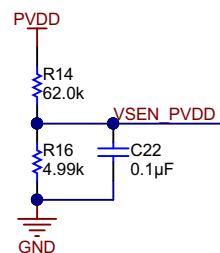
Figure 5. Voltage Sense Circuit of BoosterPack
