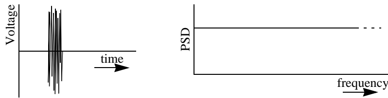
Figure 10. Impulse noise in the time and frequency domains
