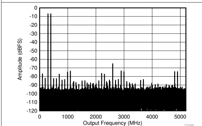
Figure 6-9. DES Mode: Single Tone FFT at 5597 MHz
