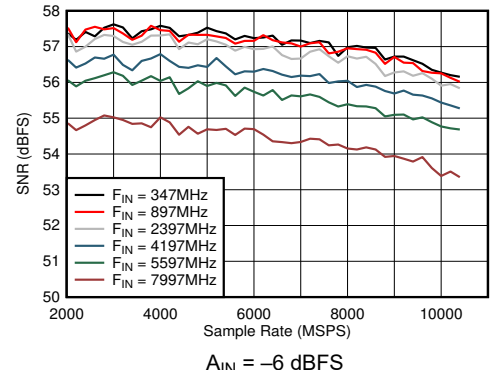
Figure 6-30. DES Mode: SNR vs Sample Rate and Input Frequency A_{IN} = -6\text{ dBFS}
