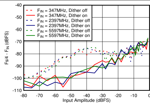
Figure 6-72. DES Mode: F_{s/4} - F_{\text{IN}} vs Input Amplitude and Dither
