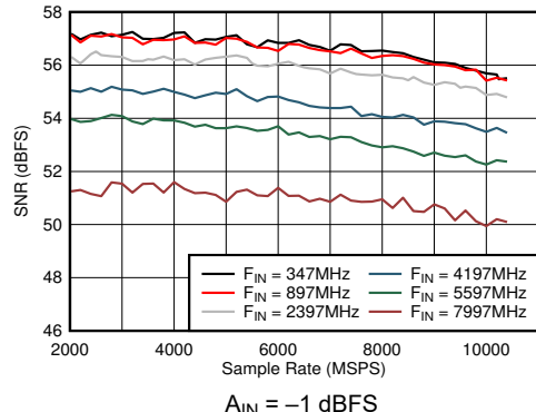
Figure 6-29. DES Mode: SNR vs Sample Rate and Input Frequency A_{IN} = -1\text{ dBFS}
