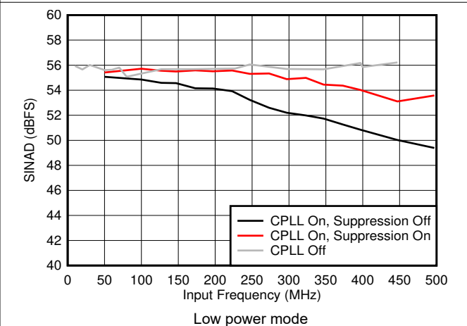
Figure 5-46. SINAD vs F_{IN} and C-PLL modes
