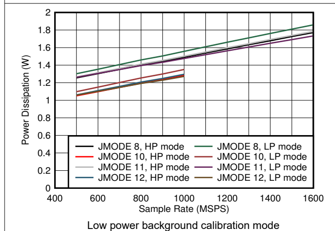
Figure 5-91. Dual Channel, Power Dissipation vs F_S and JMODE 8 - 12
