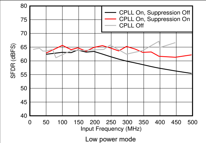
Figure 5-44. SFDR vs F_{IN} and C-PLL modes
