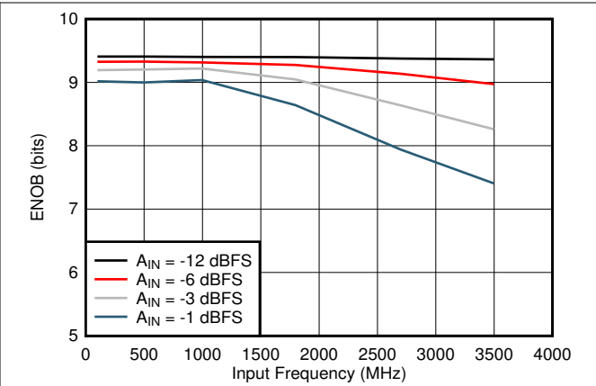
Figure 5-20. ENOB vs Input Frequency
