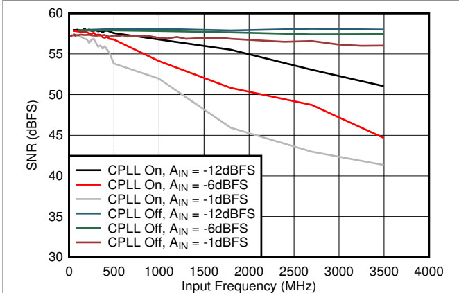
Figure 5-49. SNR vs A_{IN} and C-PLL
