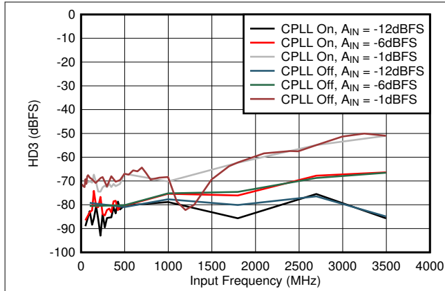
Figure 5-53. HD3 vs A_{IN} and C-PLL
