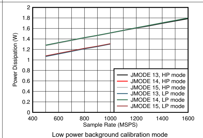
Figure 5-92. Dual Channel, Power Dissipation vs F_S and JMODE 13 - 15
