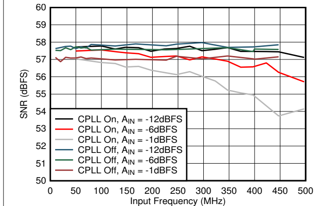
Figure 5-55. SNR vs A_{IN} and C-PLL
