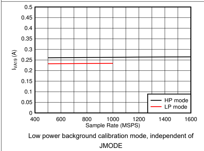
Figure 5-103. Single Channel, I_{VA19} vs F_S
