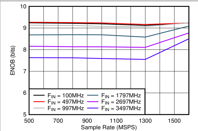
Figure 5-26. ENOB vs Sample Rate
