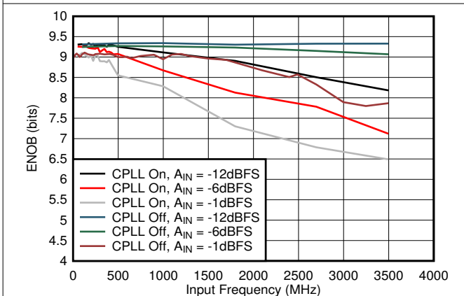
Figure 5-51. ENOB vs A_{IN} and C-PLL
