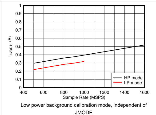
Figure 5-104. Single Channel, I_{VA11} vs F_S
