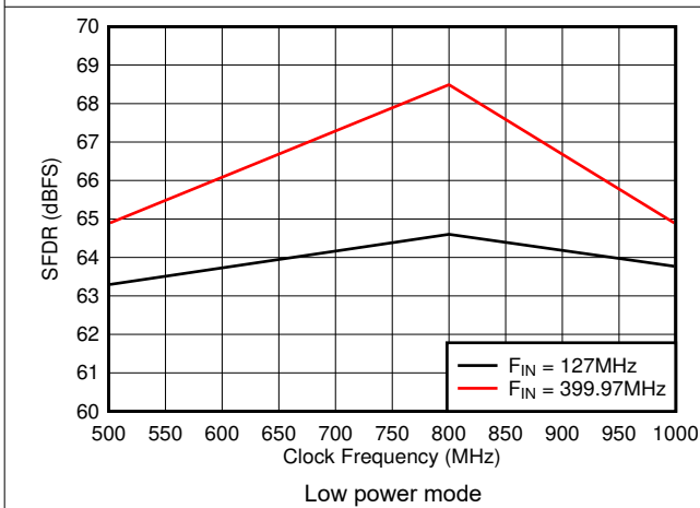
Figure 5-27. SFDR vs Sample Rate
