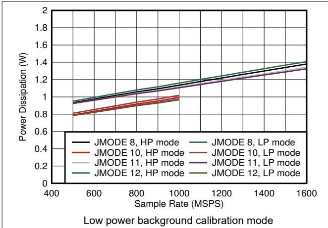
Figure 5-101. Single Channel, Power Dissipation vs F_S and JMODE 8 - 12
