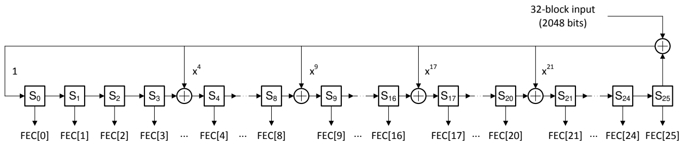
Figure 6-8. FEC Parity Bit Generator
