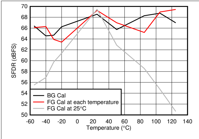
Figure 5-65. SFDR vs Temperature
