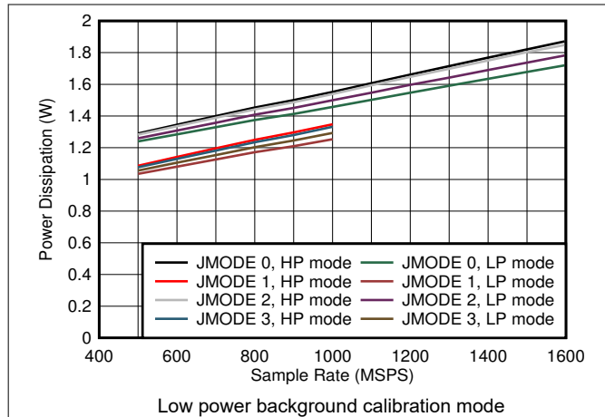
Figure 5-89. Dual Channel, Power Dissipation vs F_S and JMODE 0 - 3
