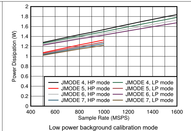
Figure 5-90. Dual Channel, Power Dissipation vs F_S and JMODE 4 - 7
