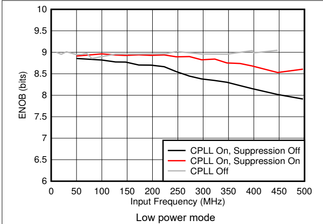
Figure 5-47. ENOB vs F_{IN} and C-PLL modes
