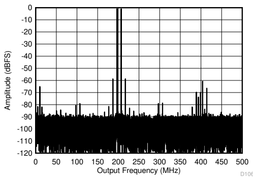
10 MHz tone spacing, -7 dBFS per tone, Low power mode, 1000MSPS Figure 5-73. Two Tone FFT at 1798 MHz
