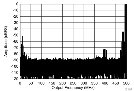
10 MHz tone spacing, -7 dBFS per tone, Low power mode, 1000MSPS Figure 5-74. Two Tone FFT at 3498 MHz
