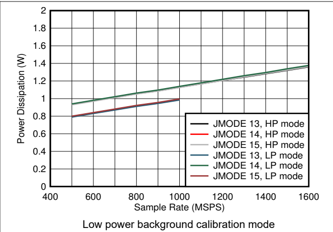
Figure 5-102. Single Channel, Power Dissipation vs F_S and JMODE 13 - 15
