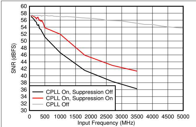
Figure 5-41. SNR vs F_{IN} and C-PLL modes
