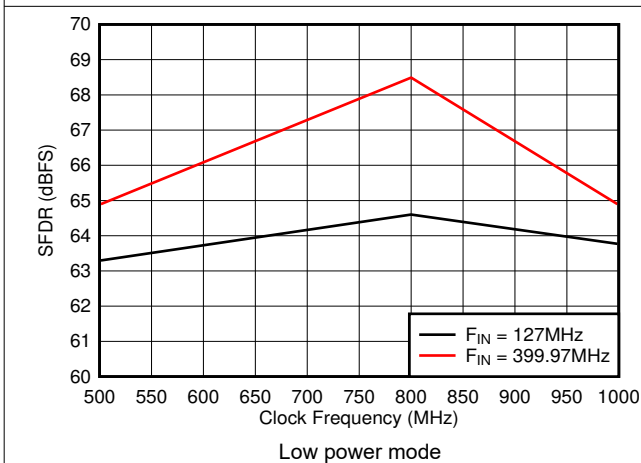
Figure 5-29. SFDR vs Sample Rate
