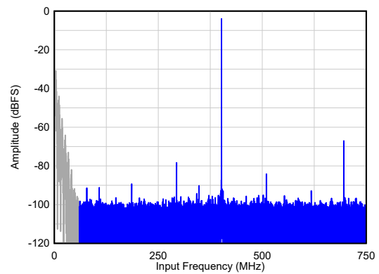
SNR = 63.4 dBFS 1 , HD23 = 63 dBc, Non HD23 = 89 dBFS A_{IN} = -4\text{ dBFS} , 1x AVG, Dither = EN
