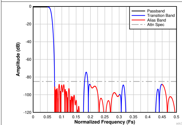
Figure 7-23. Complex Decimation by 8 Filter Response
