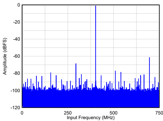
SNR = 62.6 dBFS, HD23 = 60 dBc, Non HD23 = 79 dBFS A_{IN} = -1\text{ dBFS} , 1x AVG, Dither = DIS
