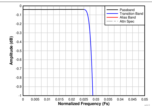
Figure 7-26. Decimation by 16 Passband Ripple Response
