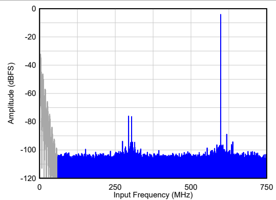
SNR = 67.0 dBFS 1 , HD23 = 72 dBc, Non HD23 = 89 dBFS A_{IN} = -4\text{ dBFS} , 2x AVG, Dither = EN
