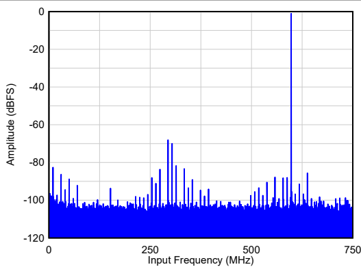
SNR = 66.8 dBFS, HD23 = 67 dBc, Non HD23 = 82 dBFS A_{IN} = -1\text{ dBFS} , 2x AVG, Dither = DIS
