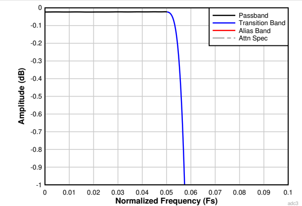
Figure 7-24. Decimation by 8 Passband Ripple Response
