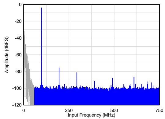
SNR = 64.1 dBFS 1 , HD23 = 71 dBc, Non HD23 = 86 dBFS A_{IN} = -4\text{ dBFS} , 1x AVG, Dither = EN
