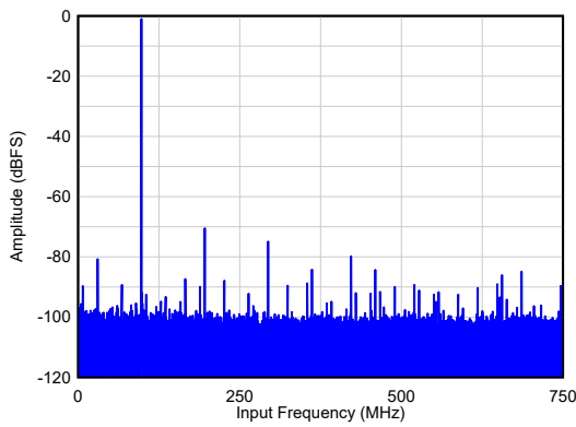
SNR = 63.8 dBFS, HD23 = 69 dBc, Non HD23 = 80 dBFS A_{IN} = -1\text{ dBFS} , 1x AVG, Dither = DIS
