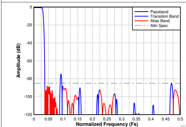
Figure 7-25. Complex Decimation by 16 Filter Response
