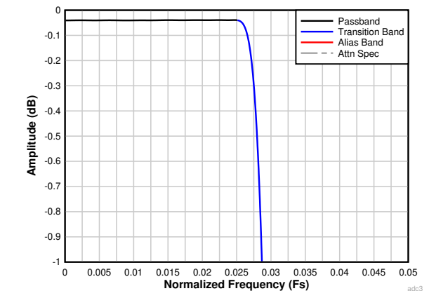
Figure 7-29. Decimation by 16 Passband Ripple Response
