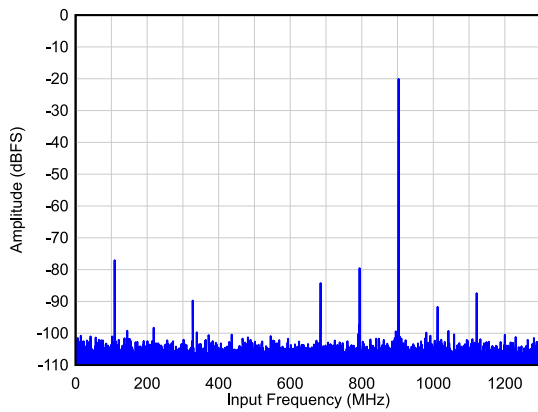
SNR = 70.0 dBFS, SFDR = 58 dBc, Non HD23 = 85 dBFS A_{IN} = -20 dBFS, 4x AVG, Dither = DIS
