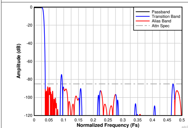
Figure 7-28. Complex Decimation by 16 Filter Response
