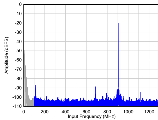
SNR = 69.5 dBFS 1 , SFDR = 67 dBc, Non HD23 = 88 dBFS A_{IN} = -20 dBFS, 4x AVG, Dither = EN
