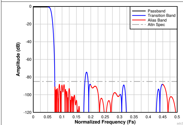
Figure 7-26. Complex Decimation by 8 Filter Response
