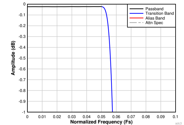
Figure 7-27. Decimation by 8 Passband Ripple Response
