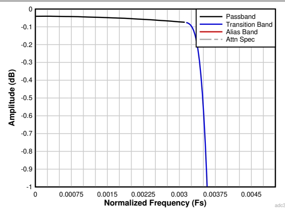
Figure 6-37. Decimation by 128 Passband Ripple Response
