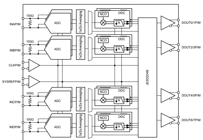
Block Diagram
