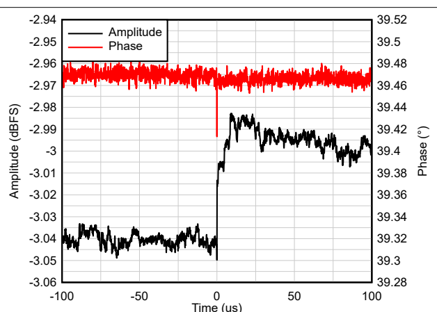
Figure 6-19. Amplitude and Phase vs Time
