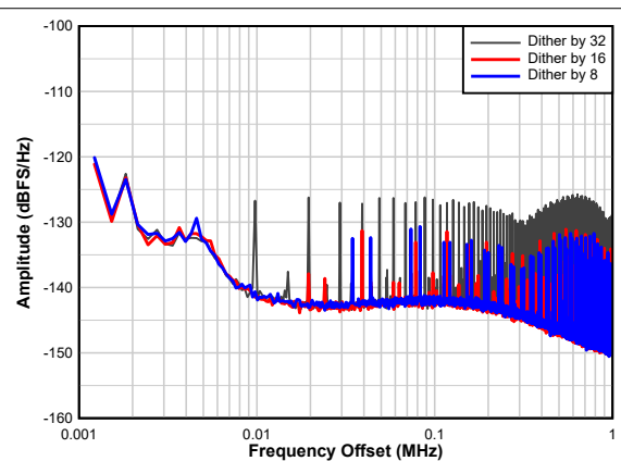
Figure 6-9. Dither vs Dither Divider Setting
