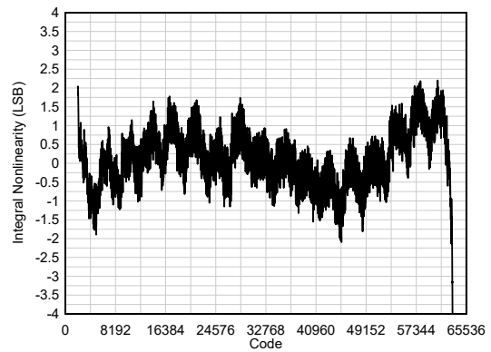
Figure 5-52. INL
