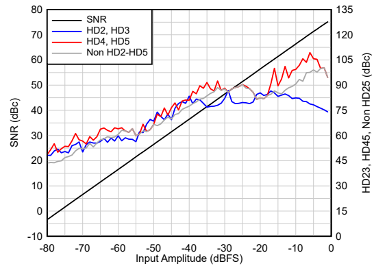
Figure 5-14. AC Performance vs A_{IN}
