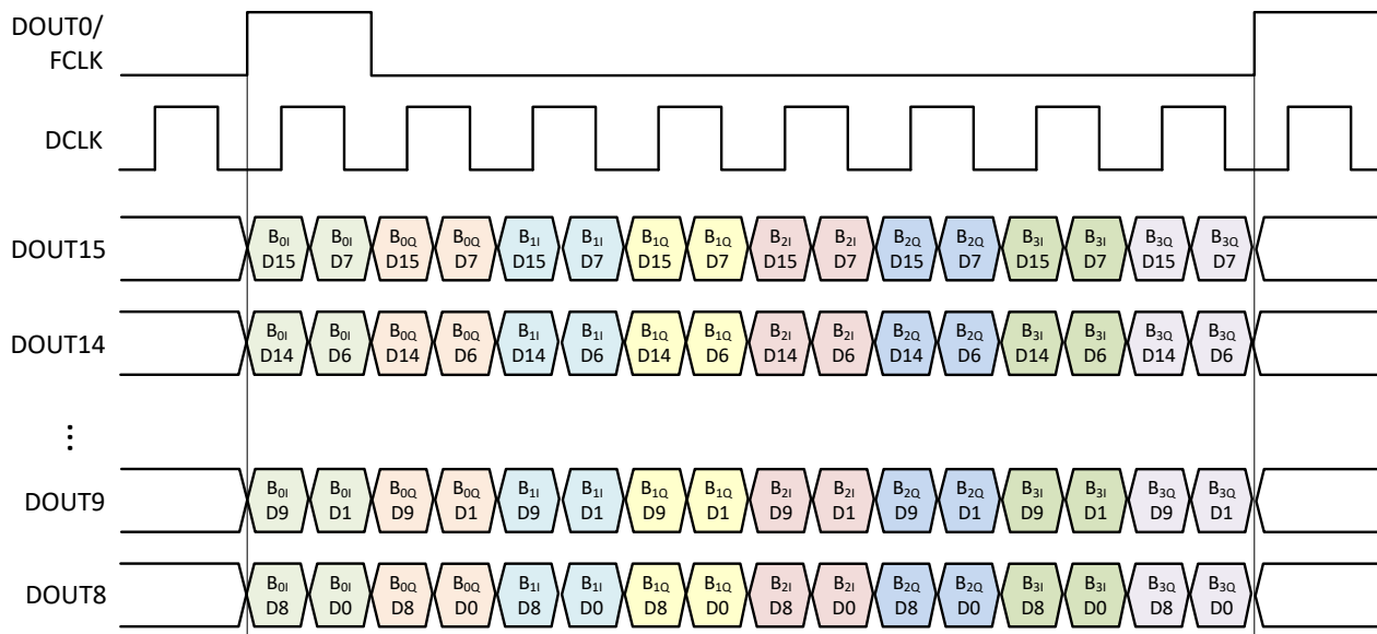
Figure 7-59. SLVDS frame assembly for example 4
