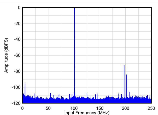
Figure 7-66. FFT: F_{IN} = 105\text{MHz} , low latency mode
