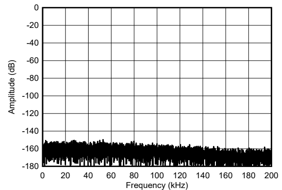
Figure 5-14. High-Speed Mode, Shorted-Input FFT
