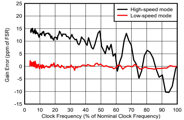
Gain error calibrated at nominal clock frequency Figure 5-56. Gain Error vs Clock Frequency
