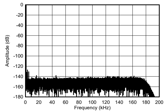
Figure 5-16. High-Speed Mode, Shorted-Input FFT
