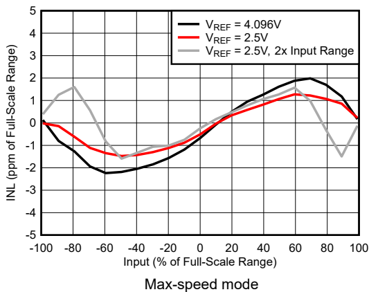
Figure 5-63. INL Error vs Input Voltage
