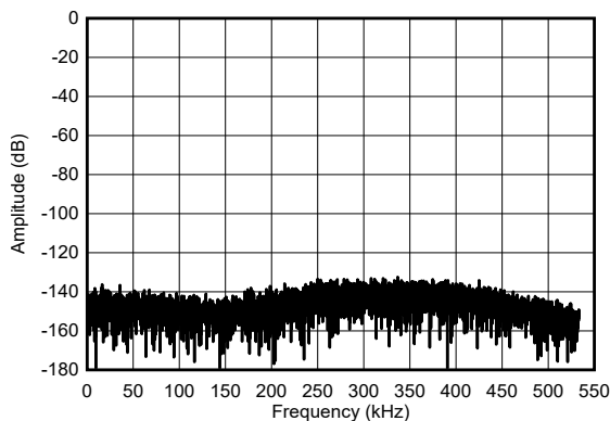
Figure 5-15. High-Speed Mode, Shorted-Input FFT
