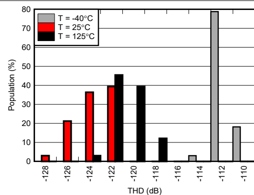
V REF = 2.5V, 30 units Figure 5-58. THD Distribution
