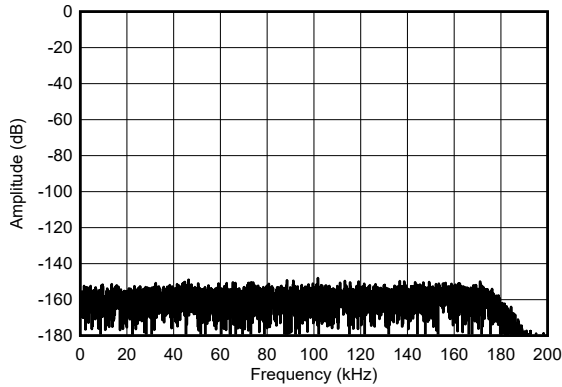
Figure 5-13. High-Speed Mode, Shorted-Input FFT
