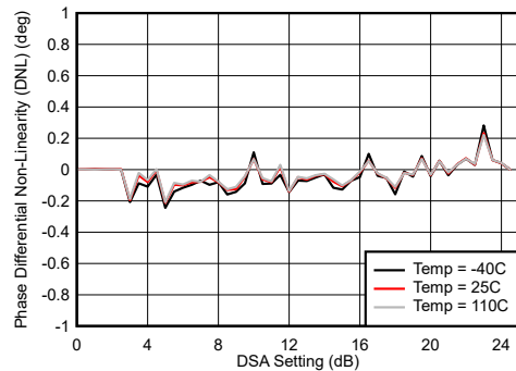
Differential Phase Error = \text{Phase}_{\text{IN}}(\text{DSA Setting} - 1) - \text{Phase}_{\text{IN}}(\text{DSA Setting}) Figure 6-6. RX Uncalibrated Differential Phase Error vs DSA Setting at 30 MHz
