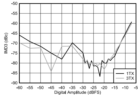
f_{\text{DAC}} = f_{\text{CLK}} = 9000 MSPS, non-interleave mode
