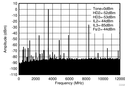
Matching at 3.5 GHz, f_{\text{DAC}} = 11.79648 \text{ GSPS} , interleave mode.
