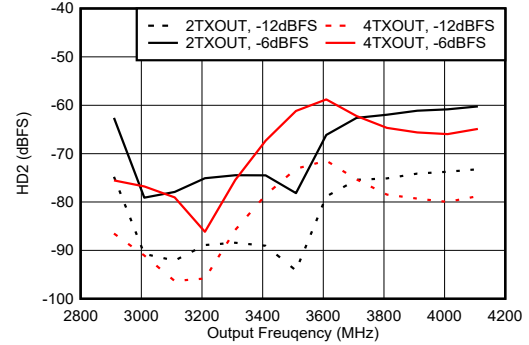
Matching at 3.5 GHz, f_{\text{DAC}} = 11.79648 \text{ GSPS} , interleave mode, normalized to output power at harmonic frequency
