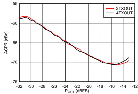
3.5 GHz Matching, single carrier 20-MHz BW TM1.1 LTE Figure 6-479. TX 20-MHz LTE ACPR vs Digital Level at 3.5 GHz
