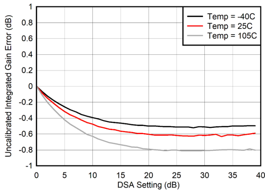
Figure 6-263. Uncalibrated TX Integrated Gain Error (INL) at 400 MHz
