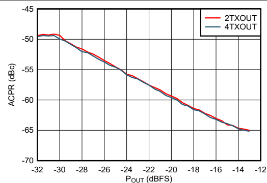
3.5 GHz Matching, single carrier 100-MHz BW NR TM1.1 Figure 6-481. TX 100-MHz NR ACPR vs Digital Level at 3.5 GHz
