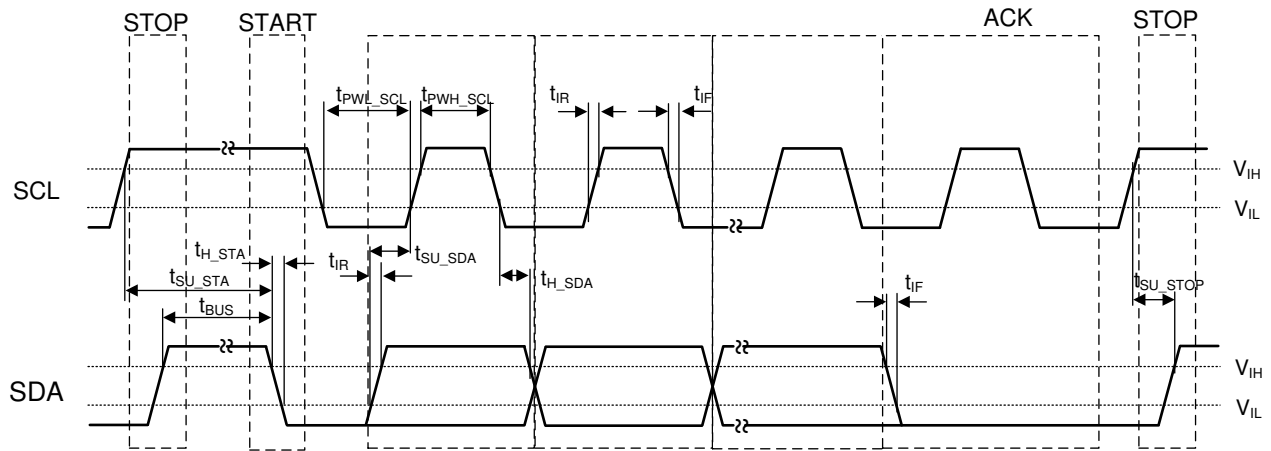
Figure 9-7. I 2 C Timing
