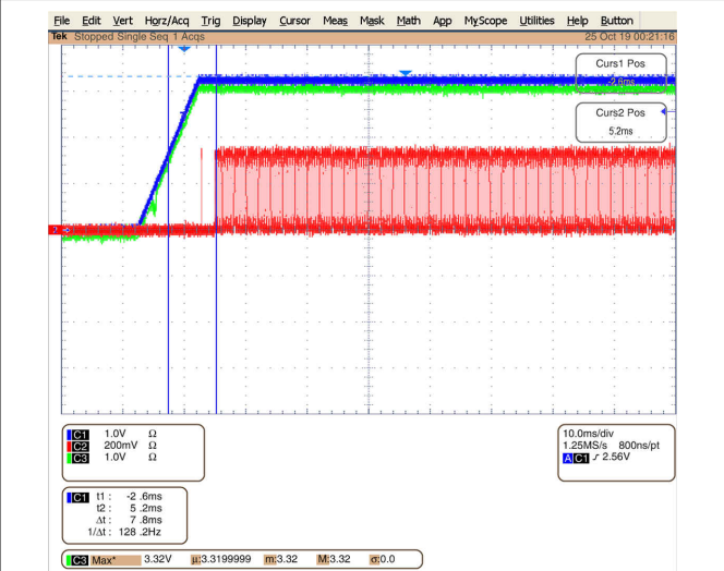
Figure 8-8. All Power Supply = 3.3 V, VDD Ramp Time = 10 ms
