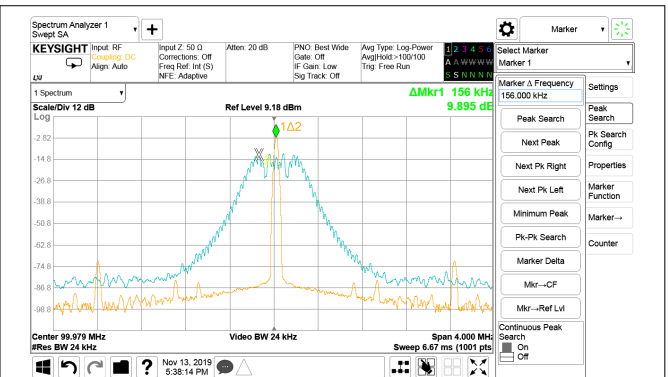
Figure 10-5. 100 MHz With ±0.25% Center Spread With and Without Trace
