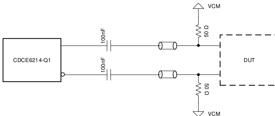
Figure 9-13. LVDS Output - AC-Coupled
