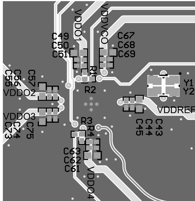
Figure 11-6. Layout Example, Bottom Layer
