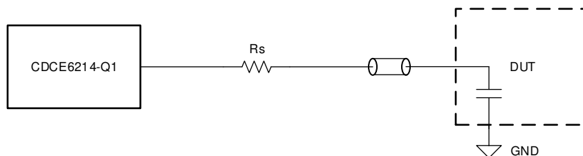
Figure 9-11. LVCMOS Output
