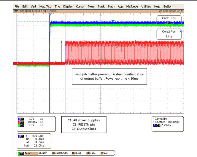
Figure 8-6. All Power Supply = 3.3 V, VDD Ramp Time = 1 ms
