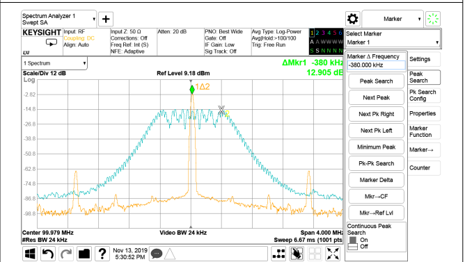
Figure 10-7. 100 MHz With ±0.5% Center Spread With and Without Trace
