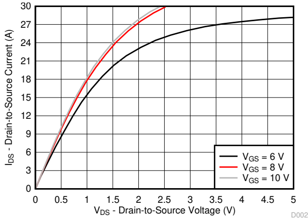
Figure 3-2. Saturation Characteristics
