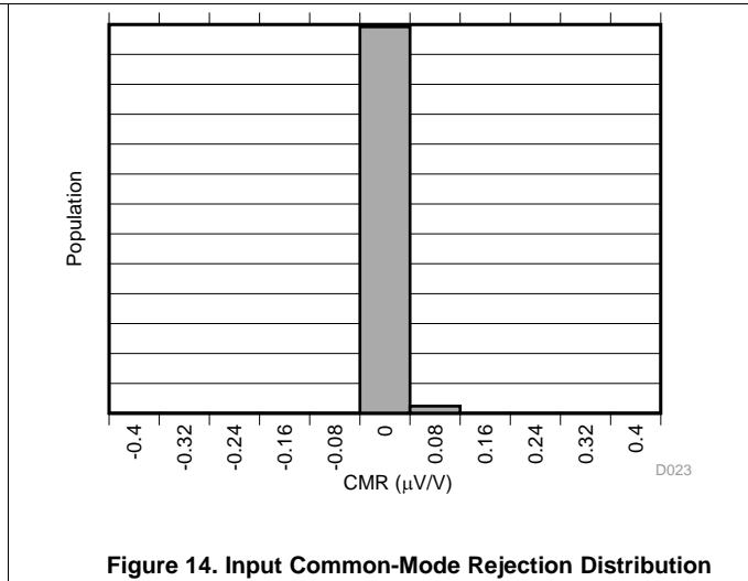
Figure 14. Input Common-Mode Rejection Distribution
