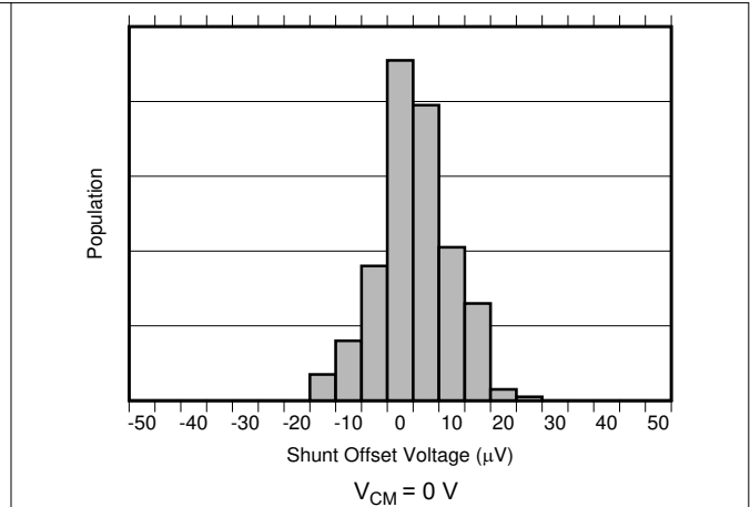
Figure 6-3. Shunt Input Offset Voltage Production Distribution
