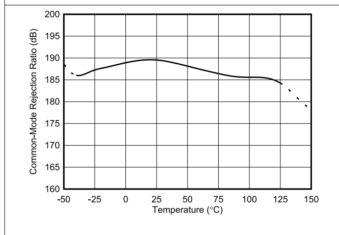
Figure 6-6. Shunt Input Common-Mode Rejection Ratio vs. Temperature
