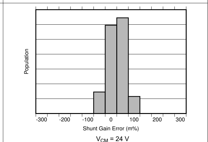
Figure 6-7. Shunt Input Gain Error Production Distribution
