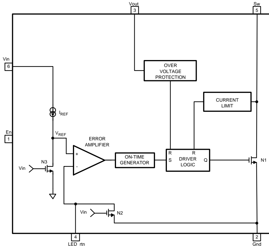
Figure 2. Block Diagram
