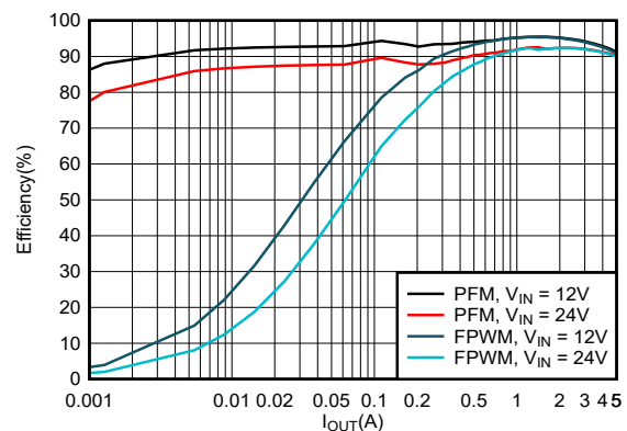
Efficiency vs Output Current V_{\text{OUT}} = 5\text{V} , 400kHz
