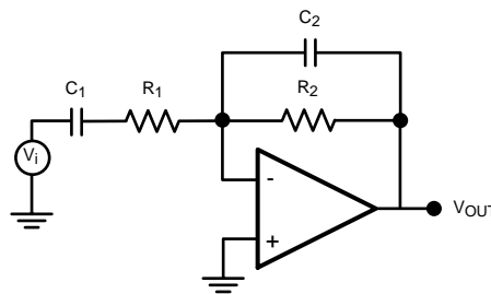
Figure 11. Bandpass Filter
