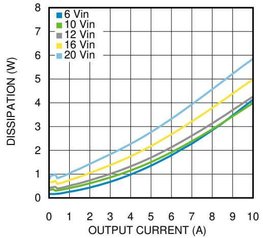
Figure 6-8. Dissipation 1.8-V Output at 25°C
