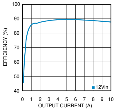
Figure 8-4. Efficiency
