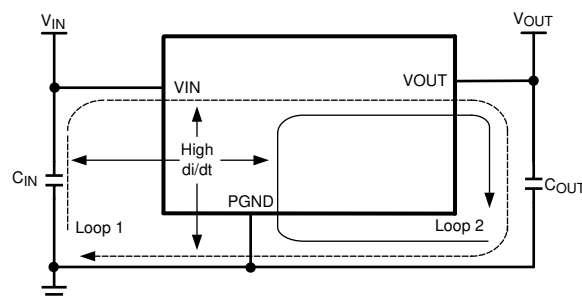
Figure 10-1. Critical Current Loops to Minimize
