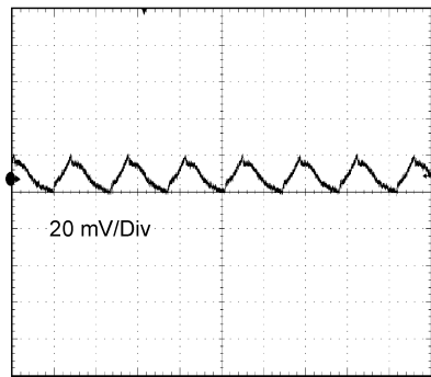
TIME (2 \mu\text{s}/\text{Div} ) 12 \text{ V}_{IN} , 3.3 \text{ V}_{OUT} at Full Load, BW = 20 MHz Figure 6-35. Output Ripple
