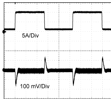
Figure 6-38. Output Ripple
