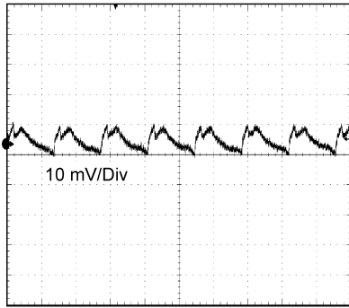
Figure 6-37. Output Ripple
