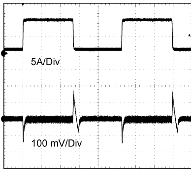
Figure 6-39. Transient Response
