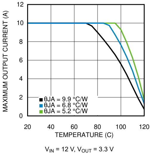
Figure 6-31. Thermal Derating
