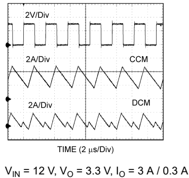
Figure 7-2. CCM and DCM Operating Modes
