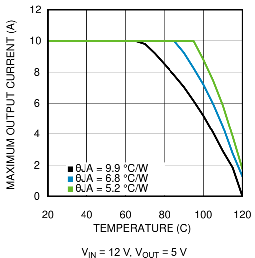
Figure 6-30. Thermal Derating
