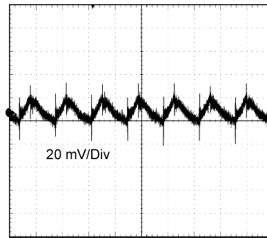
TIME (2 \mu\text{s}/\text{Div} ) 12 \text{ V}_{IN} , 3.3 \text{ V}_{OUT} at Full Load, BW = 250 MHz Figure 6-36. Output Ripple
