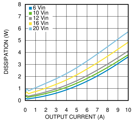
Figure 6-14. Dissipation 1-V Output at 25°C
