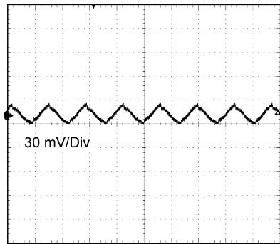
TIME (2 \mu\text{s}/\text{Div} ) 12 \text{ V}_{IN} , 5 \text{ V}_{OUT} at Full Load, BW = 20 MHz Figure 6-33. Output Ripple
