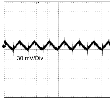
TIME (2 \mu\text{s}/\text{Div} ) 12 \text{ V}_{IN} , 5 \text{ V}_{OUT} at Full Load, BW = 250 MHz Figure 6-34. Output Ripple
