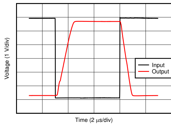
Figure 7-30. Overload Recovery
