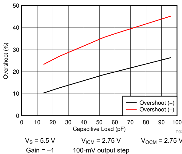
Figure 7-27. Small-Signal Overshoot vs Load Capacitance
