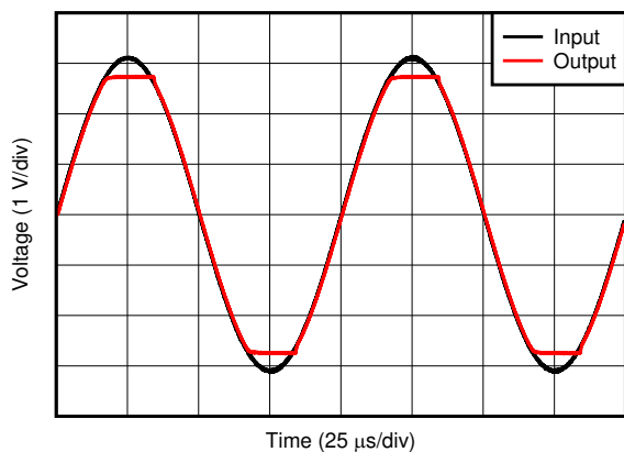
Figure 7-29. No Phase Reversal
