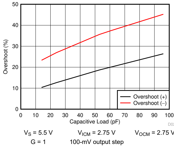
Figure 7-25. Small-Signal Overshoot vs Load Capacitance
