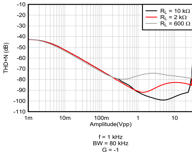
Figure 5-31. THD+N vs Output Amplitude
