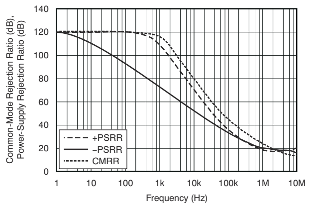
Figure 5-10. CMRR and PSRR vs Frequency (Referred-to Input)
