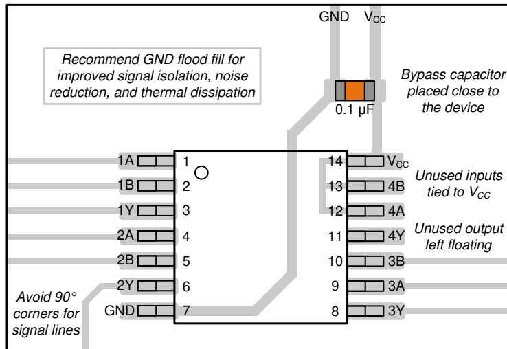
Figure 11-1. Example Layout for the SN74LV6T17-Q1
