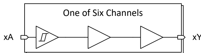
Simplified Logic Diagram (Positive Logic)
