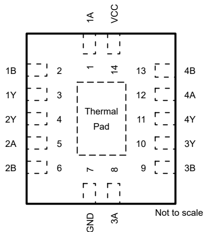
Figure 4-1. SN74LVC7266A-Q1 BQA Package, 14-Pin WQFN (Top View)
