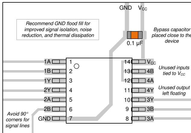
Figure 8-3. Example Layout for the SN74LVC7266A-Q1
