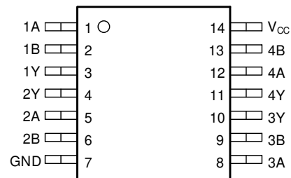
Figure 4-2. SN74LVC7266A-Q1 PW Package, 14-Pin TSSOP (Top View)
