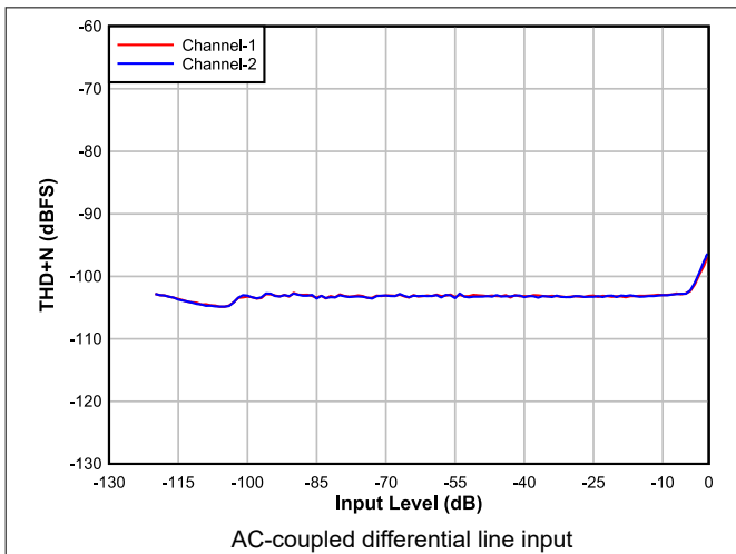
Figure 6-5. ADC THD+N Level vs Input
