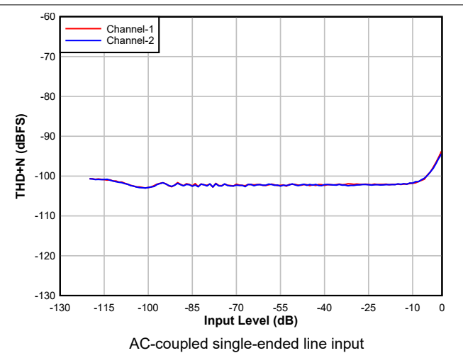
Figure 6-6. ADC THD+N Level vs Input
