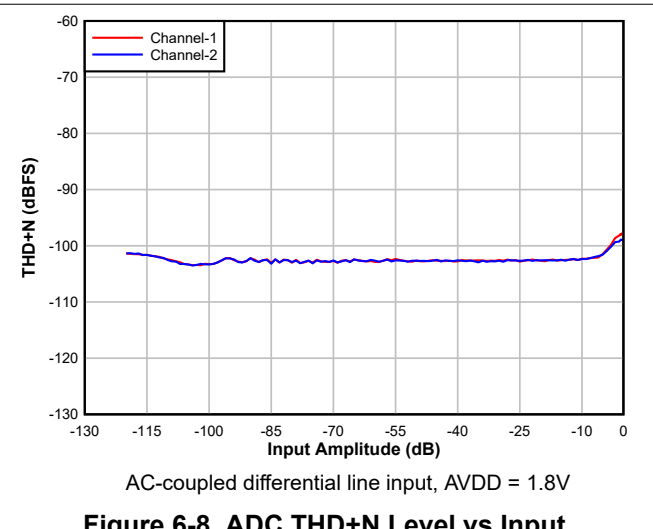
Figure 6-8. ADC THD+N Level vs Input
