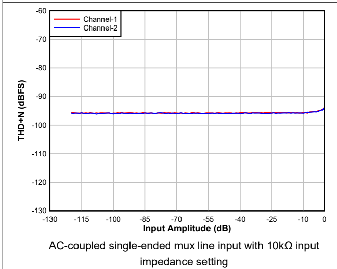
Figure 6-7. ADC THD+N Level vs Input
